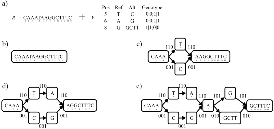
Figure. S2.3. a) The reference sequence and variant set used in graph construction. b) A graph is initialized with a single node encoding the reference sequence. c) In the order of the reference coordinate space, the variant T \rightarrow C is introduced into the graph. d) A consecutive variant (A \rightarrow G) is added to the graph. e) An insertion (G \rightarrow GCTT) is added to the graph. The final population graph encodes three paths, one of which is the reference path.
