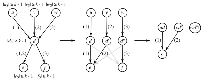
Figure. 2.9. Subgraph with haplotypes: {1,2,3}. Node d must be duplicated, as no more edges can be removed through extension or collapsing without introducing ambiguity. By grouping incoming and outgoing haplotypes on d , the number of duplications can be reduced. In the resulting graph, edges (u, d) , (v, d') , and (w, d'') can be collapsed. Finally, an extension can be applied to edges (ud, e) and (vd', e) which would lead to the null graph. Note that the introduction of grayed-out edges is prevented using haplotyping; hence the edge count is reduced from 6 to 3.
