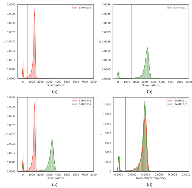
Figure. S6.2. Per-region coverage distribution plots: (a) Sample with an optimal cutoff at 500 reads. (b) Sample with an optimal cutoff at 1500 reads. (c) Both samples overlaid showing both cutoffs. (d) Both samples are overlaid with normalized frequencies showing a cutoff of 0.0001.
