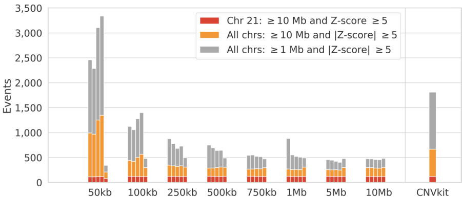
Figure. 5.1. Stacked counts of detected CNVs relative to region size and method, ordered from left to right as: WCR , WCR+SE , WCR+PE , WCR+PEI , WCRX ( CNVkit results are displayed separately). Bar coloring denotes mutually exclusive filtering constraints. Red: filtering for \geq 10 Mb CNVs with Z\text{-score} \geq 5 (only including duplications) and only on chromosome 21. Orange: filtering for \geq 10 Mb CNVs with an absolute Z\text{-score} \geq 5 (thus also including deletions) and on all chromosomes. Gray: identical to the previous but for all CNVs \geq 1 Mb.
