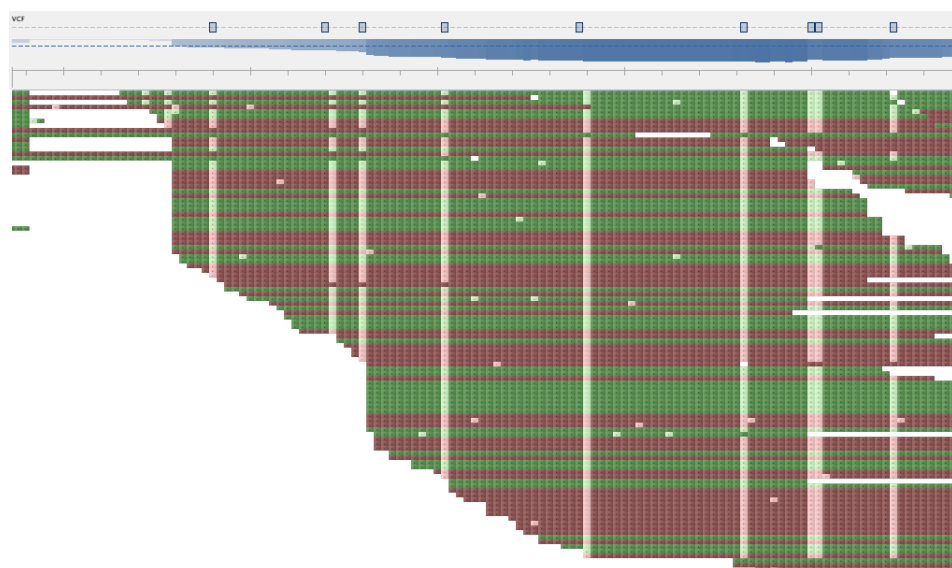
Figure. S2.19. Pileup visualization of SRR833154 reads aligned to a H37Rv graph using Tablet, with variant call annotations on top denoted as blue blocks.
