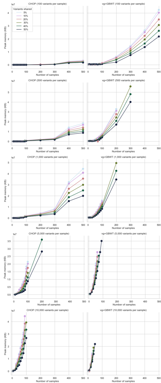
Figure. S2.17. CHOP and vg+GBWT peak memory (KB) during graph indexing for all combinations of groupings: number of variants per sample and probability of sharing variants with the population (different colors). Missing points in the plots indicate that indexing failed by exceeding one of the constraints.
