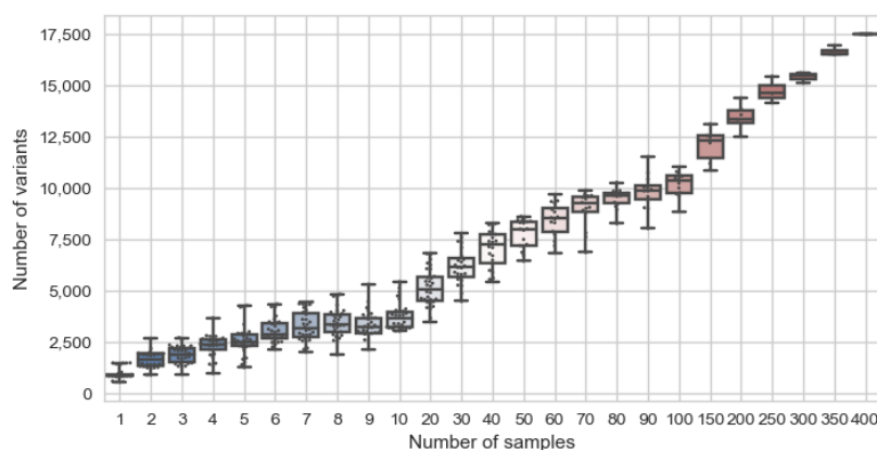
Figure. S2.2. Variable size variant sampling for VCF-based graph construction.
