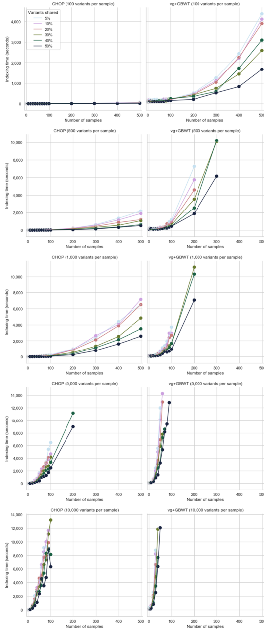
Figure. S2.16. CHOP and vg+GBWT indexing time (seconds) of the graphs for all combinations of groupings: number of variants per sample and probability of sharing variants with the population (different colors). Missing points in the plots indicate that indexing failed by exceeding one of the constraints.
