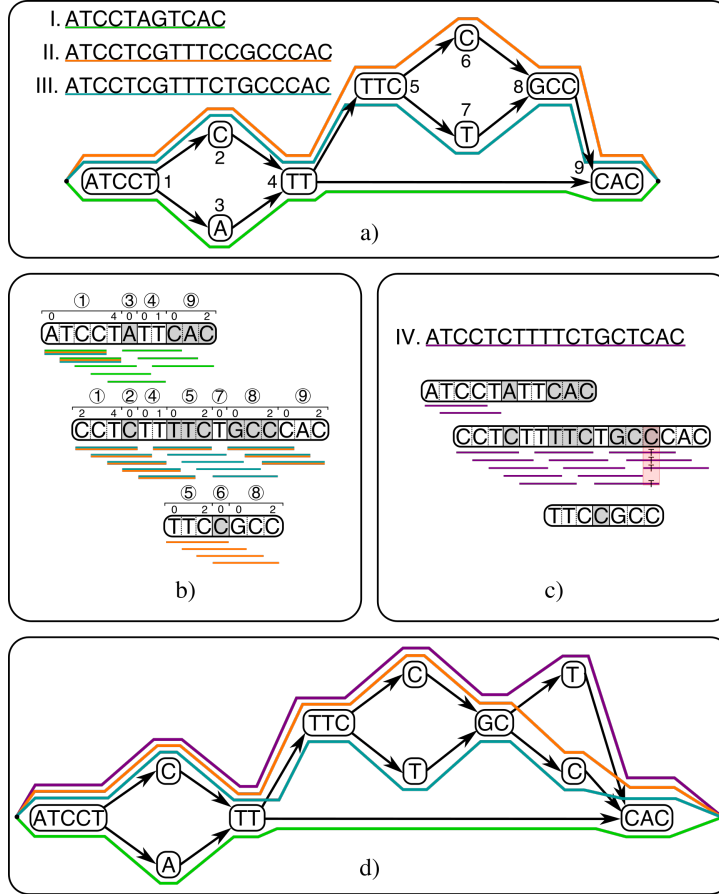
Figure. 2.1. Schematic overview of how CHOP facilitates reads alignment on a population graph. a) As input, CHOP accepts a graph representation of three distinct haplotypes (I, II, III). The colored paths through the graph identify the underlying haplotypes. b) CHOP decomposes the graph into a null graph (an edgeless graph) for substrings of length 4 (Supplemental Figure S2.1 gives all the details about the decomposition). The resulting null graph contains three nodes, and the sequence defined on these nodes covers all the substrings of length 4 that appear in the haplotypes encoded in the graph. The annotations above each node refer to intervals within nodes of the input graph. c) The reads (of length 4) from a new haplotype (IV) can be aligned to the null graph. Consequently, a mismatch can be called from the read pileup. d) With the interval definitions assigned to the null graph, the novel variant can be positioned on node 8 of the original graph and incorporated to generate a new graph.
