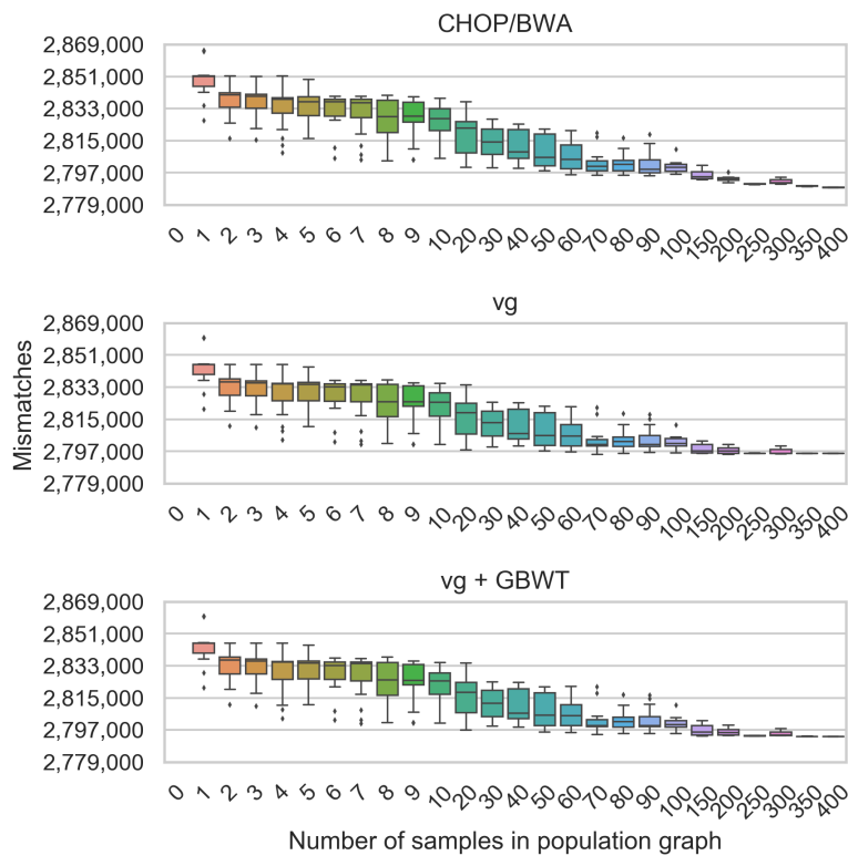
Figure. S2.8. Mismatch base count for SRR833154 alignments to different sized population graphs, containing between 0 (only H37Rv the linear reference) and 400 samples.
