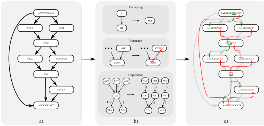
Figure. 2.6. Reporting the haplotyped k -paths in the population graph G transforms it into the null graph G^E , here k = 4 . a) A population graph with sequence encodings on the nodes. b) Indexing of k -paths based on three operations; Collapsing, merging adjacent nodes. Extension, assigning k -length substrings as prefixes or suffixes between adjacent nodes. Duplication, copying of nodes, and redistribution of edges among copies. c) The null graph encodes all 4-length paths in the original graph, coloring of lines and text denote the origin of assigned prefixes (green) and suffixes (red) (note that colored lines are not edges in the graph).
