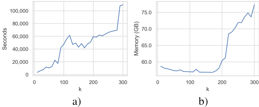
Figure. S2.14. CHOP is being measured on a population graph of human chromosome 6, for increasingly larger values of k : a) indexing time; b) peak memory in GB.
