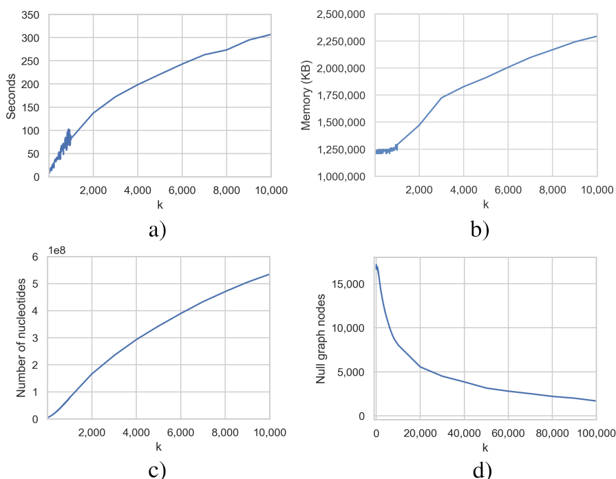
Figure. S2.13. Measurements of CHOP being run on an MTB graph ( n=401 ) for increasingly larger values of k : a) indexing time; b) peak memory in KB; c) nucleotides encoded in the null graph; d) the number of nodes in the null graph.
