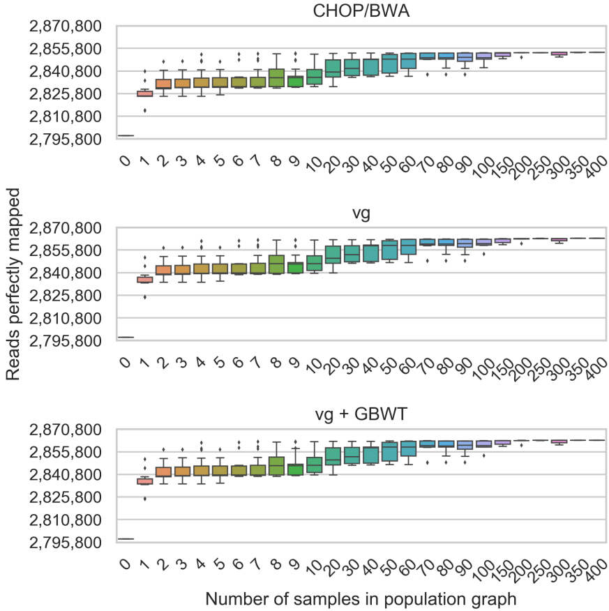
Figure. 2.2. Perfectly aligned read count for SRR833154 alignments to different sized population graphs, containing between 0 (only H37Rv, the linear reference) and 400 samples for both, when using CHOP/BWA and vg with and without haplotyping to align reads to the graph.
