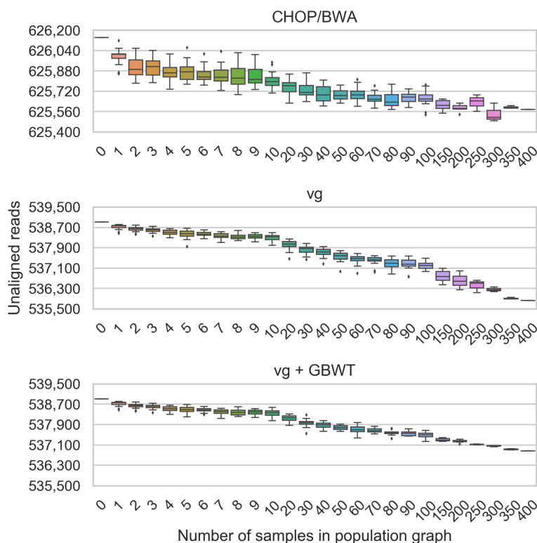
Figure. S2.7. Unaligned read count for SRR833154 alignments to different sized population graphs, containing between 0 (only H37Rv the linear reference) and 400 samples.
