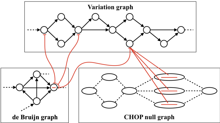
Figure. S2.20. Multiple positions in the variation graph can map to the same position in a de Bruijn graph index, while CHOP ensures a unique mapping for each.
