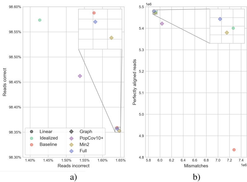
Figure. S2.12. Alignment statistics of the NA12878 simulation. a) The fraction of correctly aligned reads and incorrectly aligned reads. b) Sensitivity metrics of perfectly aligned reads and the number of mismatches.
