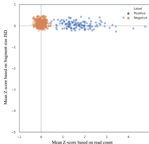
Figure. S6.7. The average Z-score of all regions (1 Mb region size) on chromosome 21 for all 526 samples for \text{WcrFF}^{\text{RC}} compared to \text{WcrFF}^{\text{FS-JSD}}
