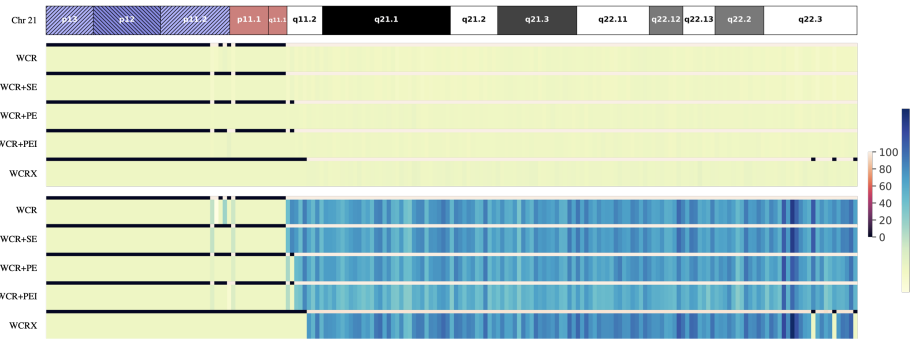
Figure. 5.2. Heatmaps of the summed per region Z\text{-scores} across all negative (top) and all T21 positive (bottom) samples at a 250 kb region scale for chromosome 21 and all different Wisecondor-based methods. The line above each method's heatmap corresponds to the average number of selected reference regions for each region of that method (black denoting that no similar reference regions are found and consequently these regions are excluded).
