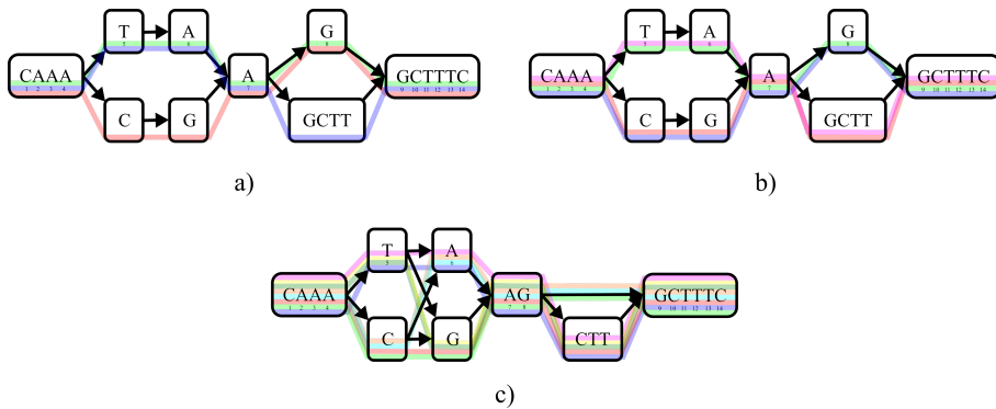
Figure. S2.5. The graph construction strategy of CHOP and vg (details in Figure S2.4) can affect the resultant paths that are indexed. a) CHOP extracts three paths from the CHOP constructed graph. b) If the same graph is indexed by vg, there will be four paths. c) The vg constructed graph indexed by vg has eight paths.
