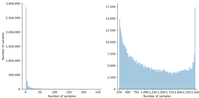
Figure. S2.9. Two histograms display the extent of shared variations among samples in the 1000 Genomes Phase 3 data of chromosome 6.
