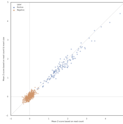
Figure. S6.4. The average Z-score of all regions (1 Mb size) on chromosome 21 for all 526 (positive and negative) samples comparing \text{WcrFF}^{\text{RC}} and \text{WcrFF}^{\text{RC}\&\text{FSmedian}} .
