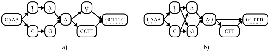
Figure. S2.4. Graph construction with the same input genome and variants as in Figure S2.3. a) Graph construction using CHOP. b) Graph construction with vg construct.
