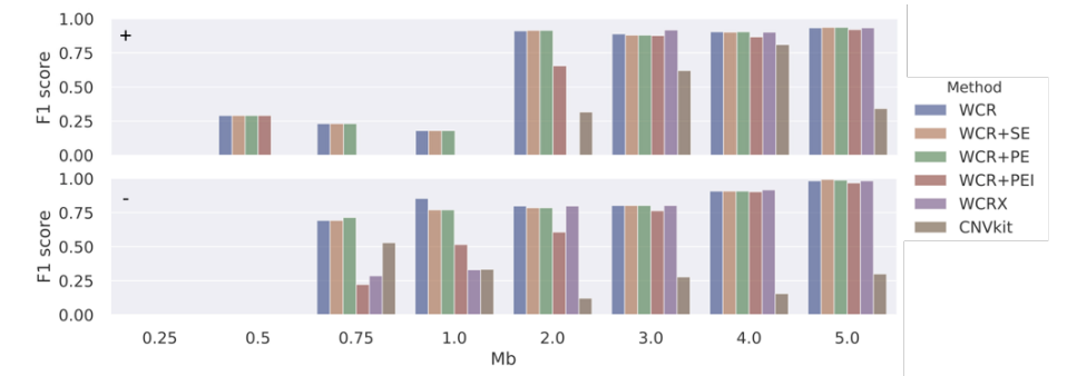
Figure. 5.5. F1 score for simulated duplication (+, top panel) and deletion (-, bottom panel) events of varying sizes (0.25 to 5 Mb) at a fixed fetal fraction of 6% for the different methods using a 250 kb region size.
