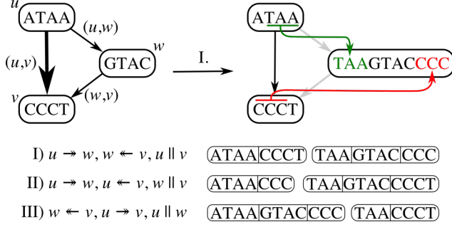
Figure. 2.8. Subgraph in which substring extension for k = 4 between (u, v) is not allowed unless either (u, w) or (w, v) are resolved first. Three distinct solutions can resolve this subgraph, and each solution is equivalent in k -path space.
