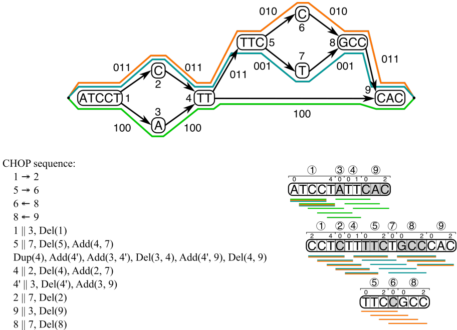
Figure. S2.1. The same graph as in Figure 2.1a is now shown with haplotypes on the edges encoded as bit vectors. Using CHOP, the input graph can be transformed into a null graph. Each of the steps performed by CHOP are shown in sequential order; Extension: x \rightarrow y ( y is prefixed by x ), and x \leftarrow y ( x is suffixed by y ). Collapsing: x||y ( x and y are collapsed into a single node). Duplication: \text{Dup}(x) , (node x is duplicated).
