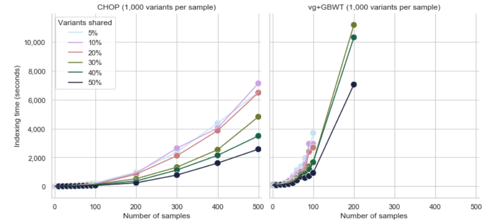
Figure. 2.3. CHOP and vg+GBWT indexing time (seconds) of graphs with increasing numbers of encoded samples, where each sample contributes 1,000 variants to the graphs. The coloring indicates different probabilities of sharing variants within the simulated population. For instance, with a probability of 5%, 95% of all sample variation will be unique to that particular sample, while the remainder is shared with one or more other samples. Missing dots in the plots indicate that the indexing failed by either exceeding 4 hours of computation time or the maximum memory of 80 GB. More details can be found in Supplemental Section 2.5.17.
