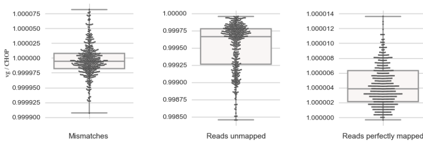
Figure. S2.6. SRR833154 graph alignments with vg using graphs constructed by either CHOP or vg. The y-axis represents a ratio (vg over CHOP) for the number of mismatches, unaligned reads, and perfectly aligned reads in the alignments.
