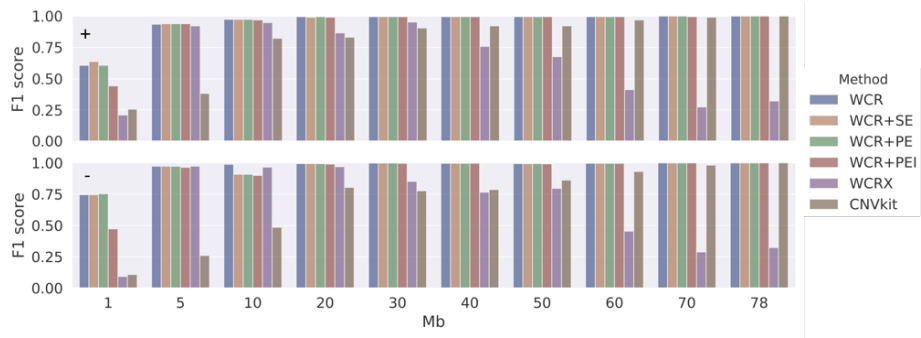
Figure. 5.4. F1 score (vertical axes) for simulated duplication (+, top panel) and deletion (-, bottom panel) events of varying sizes (1 to 78 Mb) at a fixed fetal fraction of 7.5% for the different methods using a 250 kb region size.
