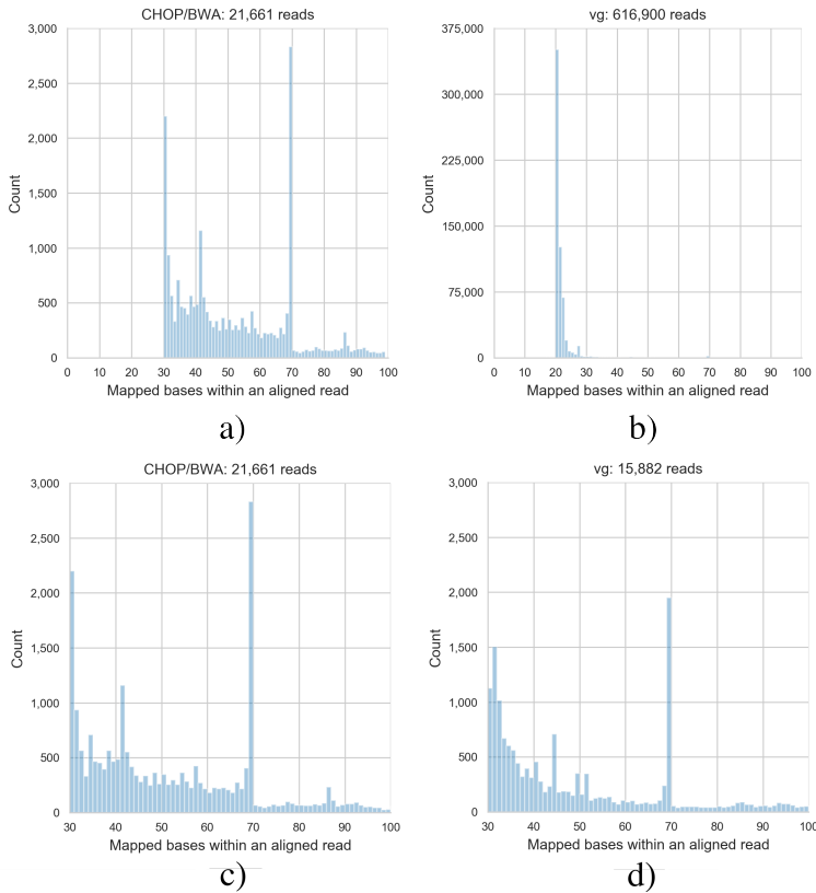
Figure. S2.10. The number of reads that have a particular number of bases aligned after their alignment onto the chromosome 6 population graph with CHOP/BWA (a) and vg (b), respectively. In c) and d), the same is shown in the range of 30 to 100 bases.
