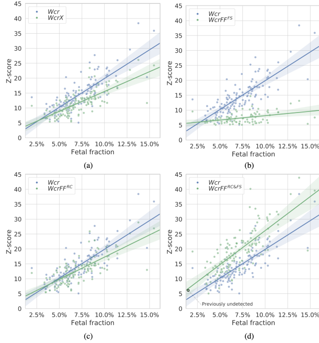
Figure 6.4. Z-scores of duplication events on chromosome 21 (an event is detected when a segment is larger than 10 Mb with a Z-score \geq 5 ) as detected by the different methods in the 125 T21 samples with respect to the estimated fetal fractions of each sample. In each panel one of the methods is compared with WCR (in blue): (a) WcrX, (b) WcrFF FS , (c) WcrFF RC , and (d) WcrFF RC&FS (all in green). The region size was 750 kb. Each point corresponds to an event within a sample.
