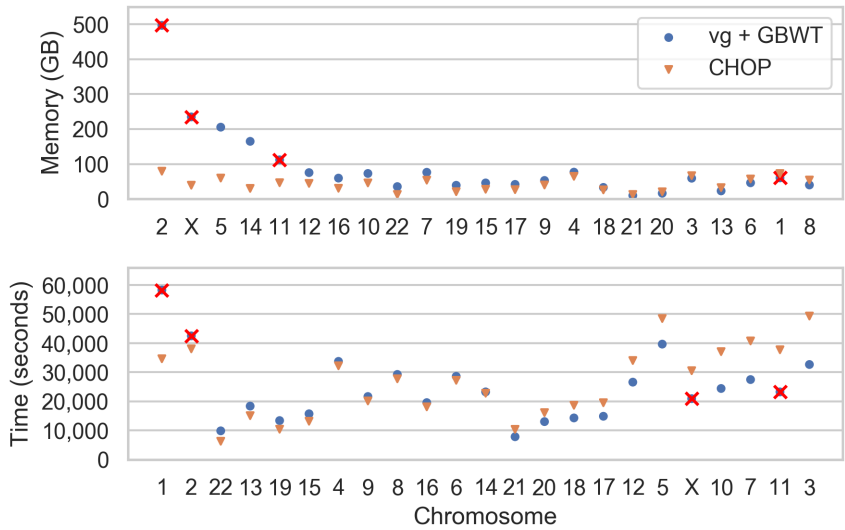
Figure. 2.4. Peak memory footprint and time required for indexing the human chromosomes using CHOP and vg+GBWT. Chromosomes are ordered according to the relative differences between CHOP and vg+GBWT. Chromosomes 1, 2, 11, and X are crossed out for vg, given that these exceeded the memory (>500 GB) or disk space (>6 TB) constraints.
