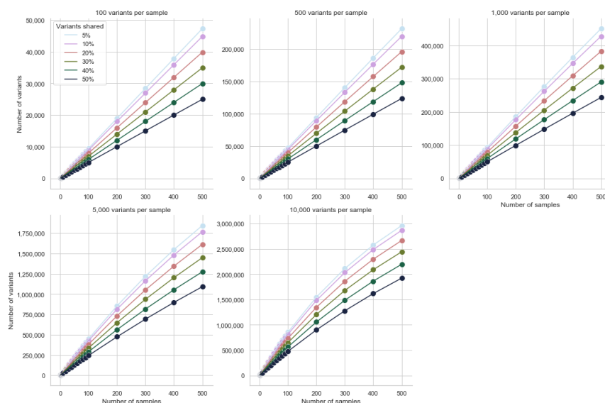
Figure. S2.15. The number of variants encoded in merged VCF files for all combinations of groupings: number of variants per sample (different plots) and probability of sharing variants with the population (different colors).
