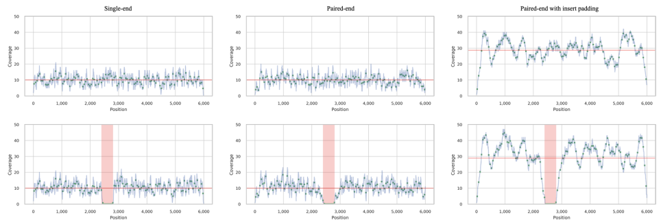
Figure. S5.2. Simulated read alignment counts across a small genome of single-end, paired-end, and paired-end with insert padding methods. On top this is shown for an unaffected sample, and on the bottom for a sample with a 400 bp deletion.
