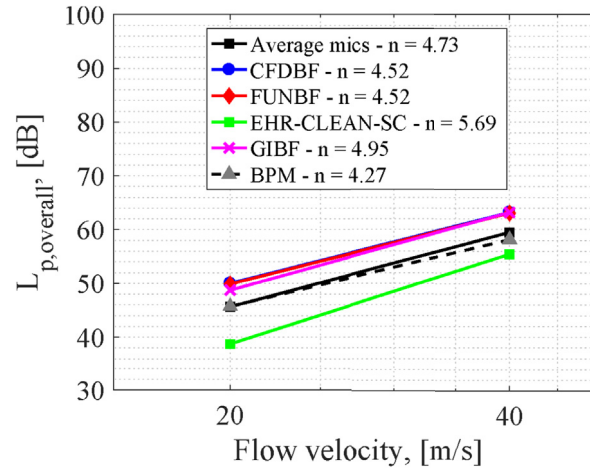
Fig. 17. Dependence between the overall trailing-edge noise levels (between 500 Hz and 5 kHz) and the flow velocity for all the acoustic imaging methods considered for the NACA 0018 airfoil, as well as for the average microphone and the BPM method. Note the logarithmic scale in the velocity axis.
