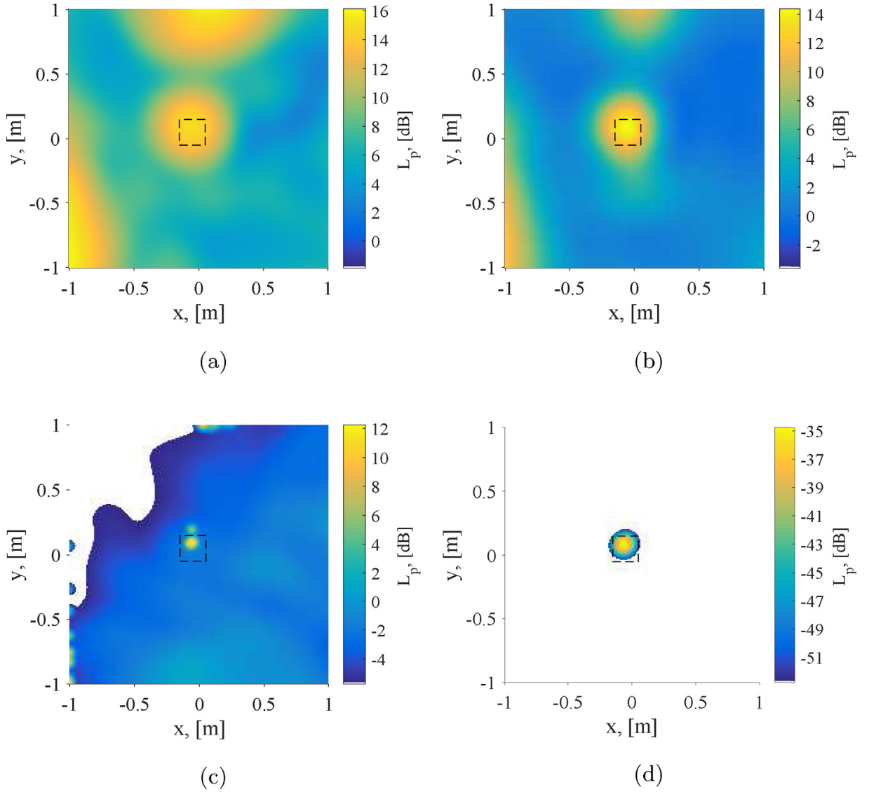
Fig. 4. Source maps for the case of a single speaker with the lowest SNR ( \text{SNR}_4 ) for a one-third-octave frequency band centered at 630 Hz for: (a) CFDBF, (b) FUNBF with \nu = 8 , (c) EHR-CLEAN-SC, and (d) GIBF. The dashed squares denote the ROI.
