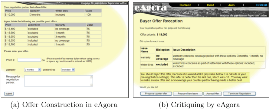
Fig. 3. The user interfaces of eAgora [13]
