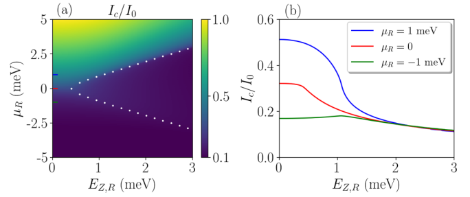
FIG. 2. Critical Josephson current in a junction between a time-reversal-invariant trivial superconductor and a Majorana nanowire lead, with an external Zeeman field E_{Z,R}\sigma_x applied only inside the Majorana nanowire. (a) I_c as a function of E_{Z,R} and \mu_R , with white dots representing the phase boundary ( E_{Z,R}^2 = \mu_R^2 + \Delta_0^2 ) of the Majorana nanowire. (b) Linecuts of I_c at fixed values of \mu_R . Here the supercurrent is due to above-gap continuum states, without any Majorana contribution. When Zeeman field is larger than the critical value ( E_{Z,R} \gtrsim \sqrt{\mu_R^2 + \Delta_0^2} ), I_c plunges with the field strength, indicating the topological quantum phase transition of the Majorana nanowire.
