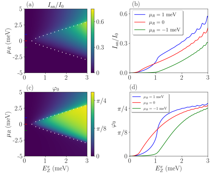
FIG. 4. Anomalous supercurrent I_{\text{an}} and phase shift \varphi_0 for the Josephson junction with a Zeeman field applied globally in the form of \vec{E}_Z \cdot \vec{\sigma} = E_Z^x \sigma_x + E_Z^y \sigma_y . The component along the spin-orbit field is fixed at E_Z^y = 0.2 \text{ meV} . (a) and (c) I_{\text{an}} and \varphi_0 as a function of \mu_R and E_Z^x . Their values in the topological regime are much larger than in the trivial regime due to the Majorana contribution. Here white dots represent the phase boundary (E_Z^x)^2 + (E_Z^y)^2 = \mu_R^2 + \Delta_0^2 . (b) and (d) Linecuts of I_{\text{an}} and \varphi_0 for fixed values of \mu_R . Note that I_{\text{an}} and \varphi_0 increase abruptly near the topological transition.
