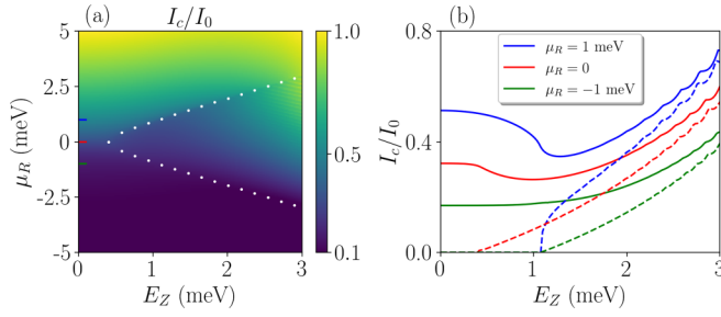
FIG. 3. Critical current in a junction between a trivial superconductor and a Majorana nanowire lead, with an external Zeeman field applied equally in both leads E_Z \sigma_x . (a) I_c as a function of E_Z and \mu_R , with white dots representing the phase boundary ( E_Z^2 = \mu_R^2 + \Delta_0^2 ) of the Majorana nanowire. (b) Linecuts of I_c at fixed values of \mu_R . Solid lines are the total critical current from both MZM and continuum states, while dashed lines are critical current due to only MZM.
