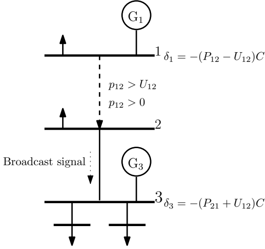
Fig. 2. Congestion detection at node 2.
