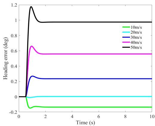
(a) Heading error with varying velocity
