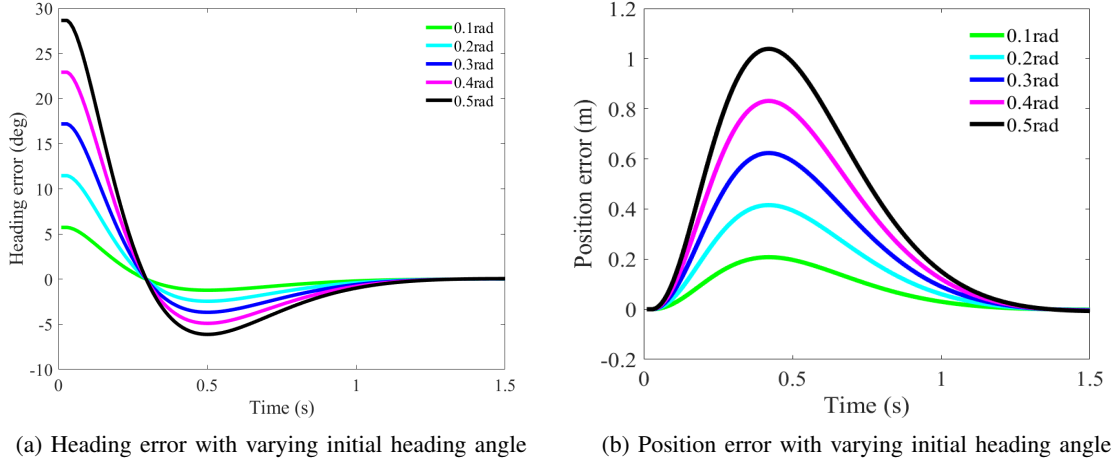
Fig. 7: Simulated steering operation during corrective steering
