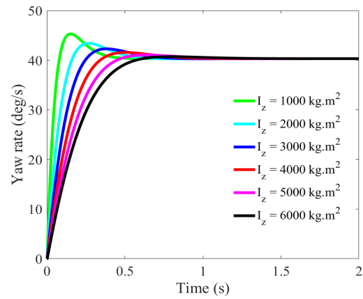
(b) Model response to varying moment of inertia
