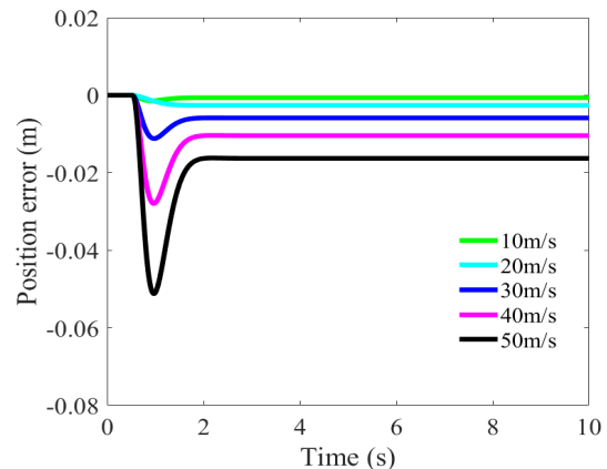
(b) Position error with varying velocity
