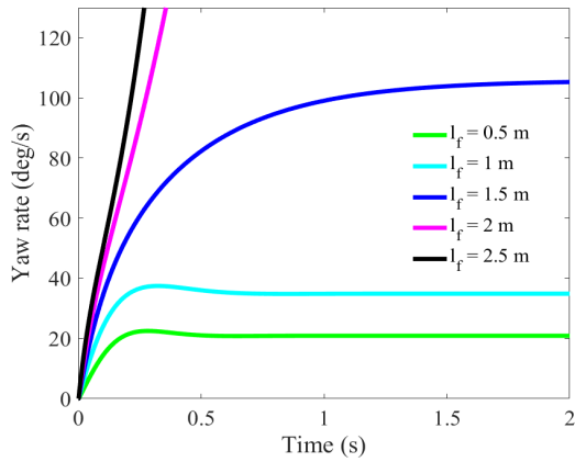
(c) Model response to shifting the center of gravity away from the front wheel
