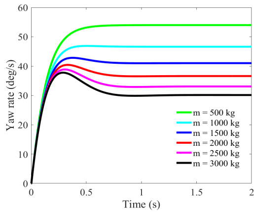
(a) Model response to varying vehicle mass
