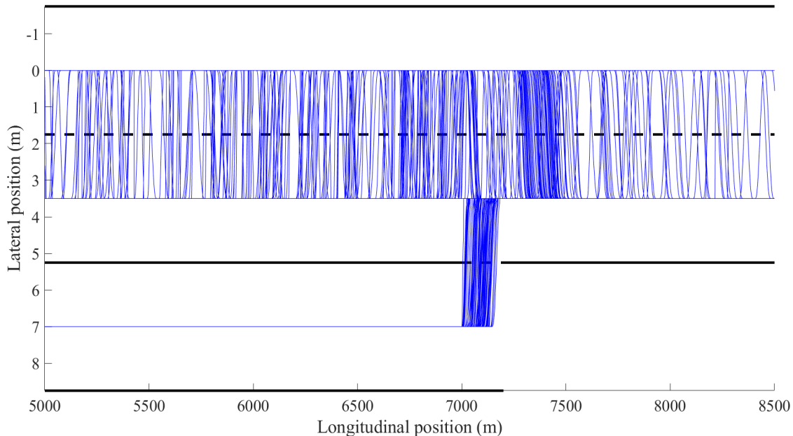
Fig. 12: Simulation results; blue lines indicate vehicle trajectories and black lines indicate lane boundaries
