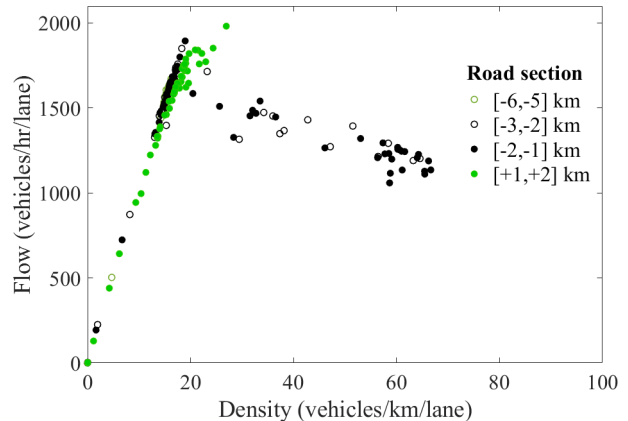
Fig. 11: Macroscopic traffic flow with varying density
