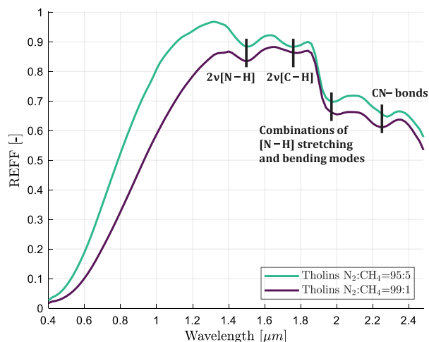
Fig. 13. Bands assignment for laboratory reflectance spectra of 5%CH 4 and 1%CH 4 tholins (geometry: i = 0^\circ , e = 30^\circ ). (For interpretation of the references to colour in this figure legend, the reader is referred to the web version of this article.)
