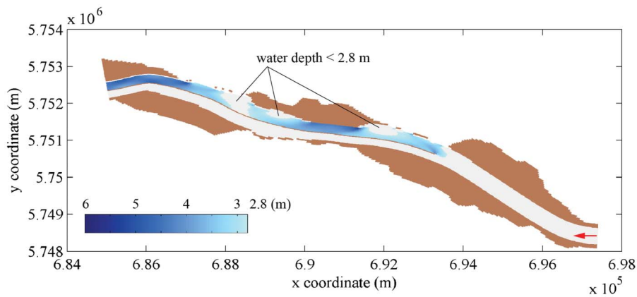
Fig. 12. Water depth at Q_{low} = 680 \text{ m}^3/\text{s} in W3 run. Flood plains and training structures are colored brown. Gray areas in the water body indicate a local water depth less than 2.8 m. Coordinates are in the Universal Transverse Mercator system.
