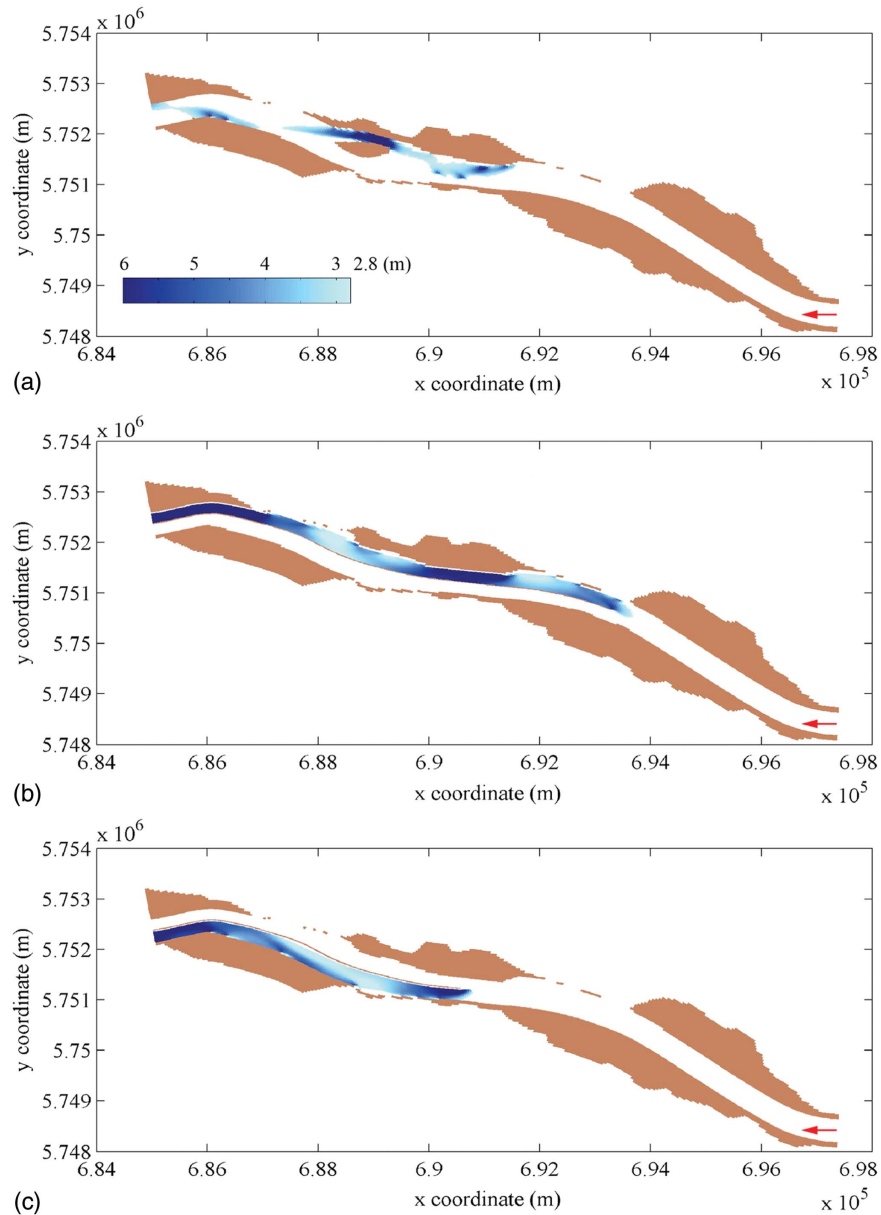
Fig. 11. Water depth distribution at low-flow ( Q_{low} = 680 \text{ m}^3/\text{s} ). Flood plains and training structures are colored brown. Gray areas in the water body indicate local water depth less than 2.8 m: (a) base-case scenario (average water depth: 1.86 m); (b) wall scenario, with wall starting upstream of point bar I top and navigation channel width equal to 200 m (average water depth: 5.13 m); (c) wall scenario with wall starting downstream of point bar I top and navigation channel width equal to 200 m (average water depth: 5.16 m); (d) groyne scenario with river-flow width of 260 m (average water depth: 3.99 m); and (e) groyne scenario with river-flow width of 200 m (average water depth: 5.17 m). The location of point bar I is indicated in Fig. 3(a). Coordinates are in the Universal Transverse Mercator system.
