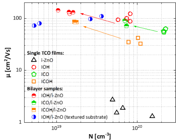
Fig. 2. Charge carrier mobility ( \mu ) and concentration ( N ) of i-ZnO, IOH, ICO, ICOH monolayers (open symbols) and bilayer designs (half open symbols) on flat and micro-textured glass substrates. The presented \mu and N values are shown after PDA treatment at 200 °C, with each mono- and bi-layer having its own annealing time optimized.
