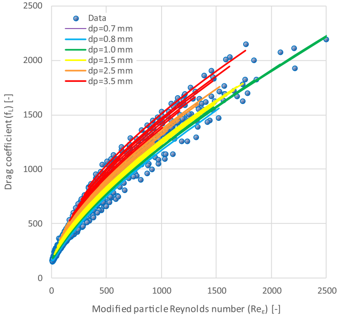
Fig. 11. Drag coefficient f_L versus Re_ε for glass beads and RIO 1 model (highest R^2 ).
