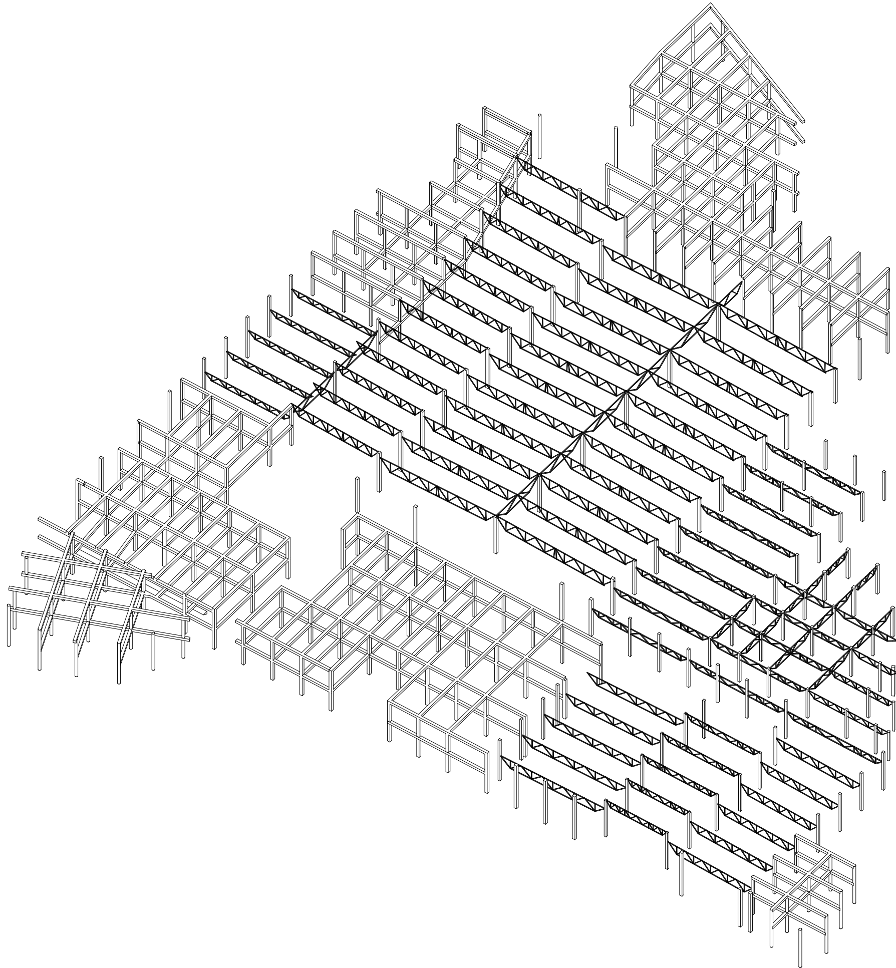
EXISTING STRUCTURE
