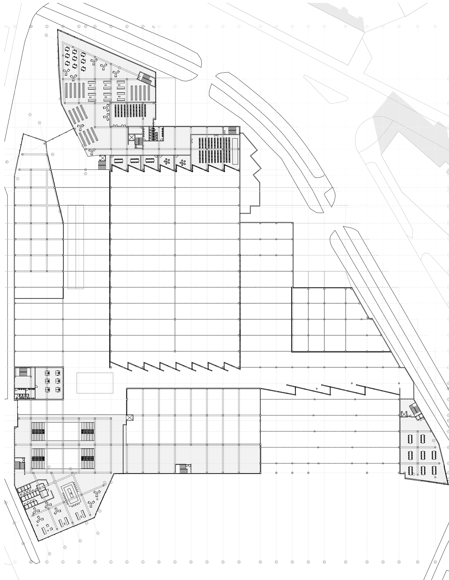
FIRST FLOOR
