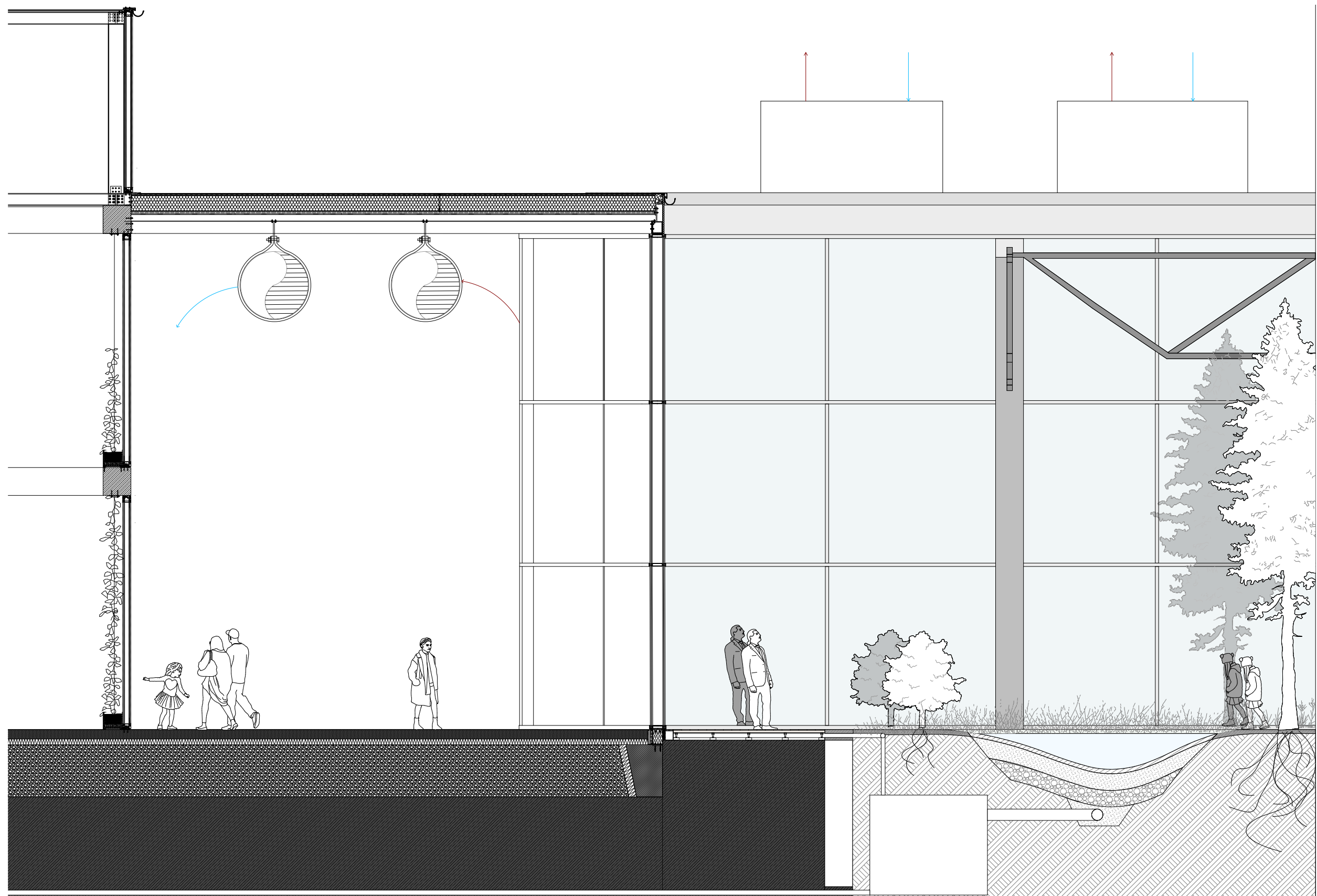
FACADE SECTION
