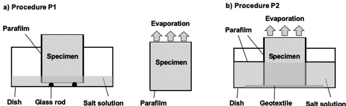
Fig. 2. Experimental setup used in the contamination experiments: (a) capillary absorption followed by drying (P1), (b) continuous capillary absorption (P2).
