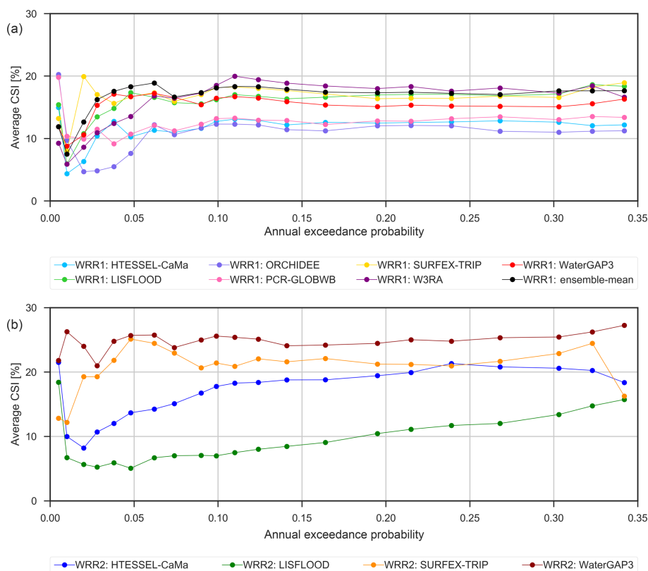
Figure 4. The critical success index (CSI) using different annual exceedance probability thresholds averaged over all gauging stations for the seven models and ensemble mean available in WRR1 (a), and the four models that are also available in WRR2 (b).
