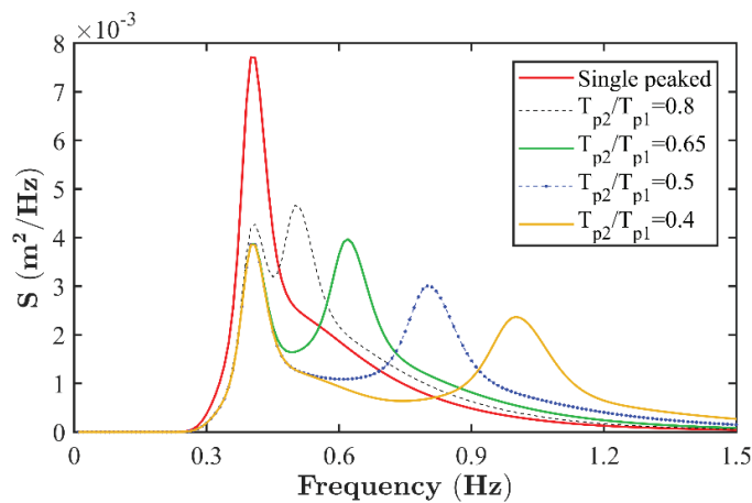
(a) Wave energy spectra with the lowest peak frequency at T_{p1} = 2.5 s.
