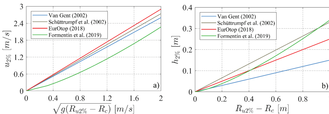
Figure 1. Comparison of existing empirical equations for a) overtopping flow velocity and b) layer thickness at smooth slopes; A slope of 1/4 was applied for calculations using EurOtop (2018) equations and Formentin et al. (2019) equations.
