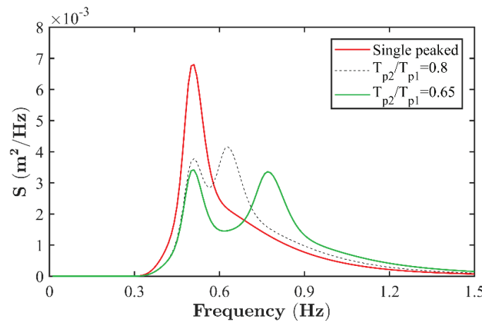
(b) Wave energy spectra with the lowest peak frequency at T_{p1} = 2.0 s.
