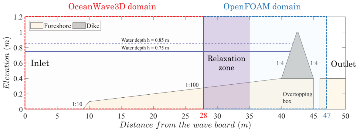
Figure 2. Set-up of the physical model in Van Gent (2002b) and numerical domain.
