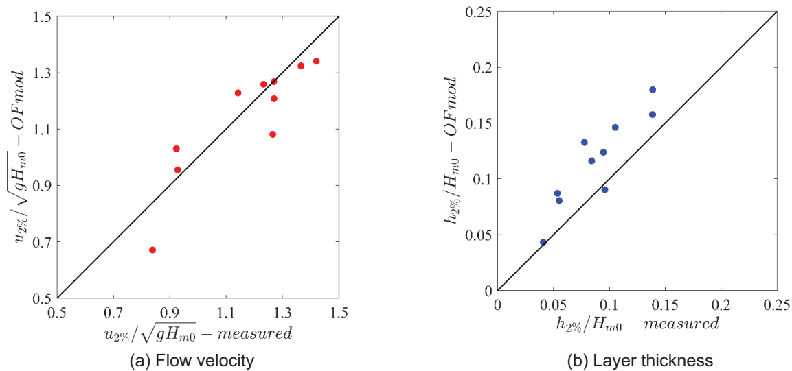
Figure 6. Comparison between the measured flow parameters and the modified flow parameters given by the OpenFOAM model taking the overestimation of wave period into account.
