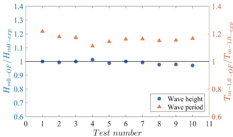
Figure 4. Comparison between modelled and measured wave characteristics significant (wave height H_{m0} and spectral wave period T_{m-1,0} ).
