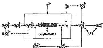
Fig. 10. Scheme for the oxidation of reduced sulphur compounds by the acidophilic thiobacilli. The boxed set of compounds and reactions represents a pool of intermediary sulphur compounds (sulphane-mono-sulphonic acids, polythionates, elemental sulphur and possibly polysulphides). The nature of the intermediary sulphur compounds formed from sulphide and elemental sulphur are unknown. Also the mechanism of sulphite formation from elemental sulphur remains to be elucidated. S_8 -sulphur may combine with polythionates to form hydrophilic sulphur complexes as shown in Fig. 6.
