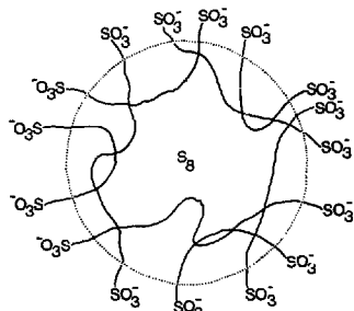
Fig. 6. Proposed structure of hydrophilic intermediary sulphur globules formed during the oxidation of tetrathionate by T. ferrooxidans . The intermediary sulphur has been demonstrated to consist of long-chain polythionates and elemental sulphur (mainly in the form of \text{S}_8 ). (Reproduced with permission from [23])
