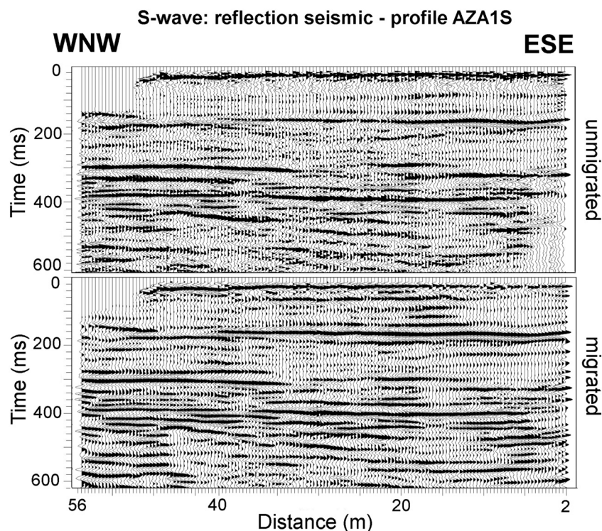
Fig. 5. Unmigrated (top) and post-stack time-migrated (bottom) stacked sections for the shallow S-wave reflection profile 1 (AZA1S), which is partially coincident with the shallow P-wave reflection profile (Fig. 4).
