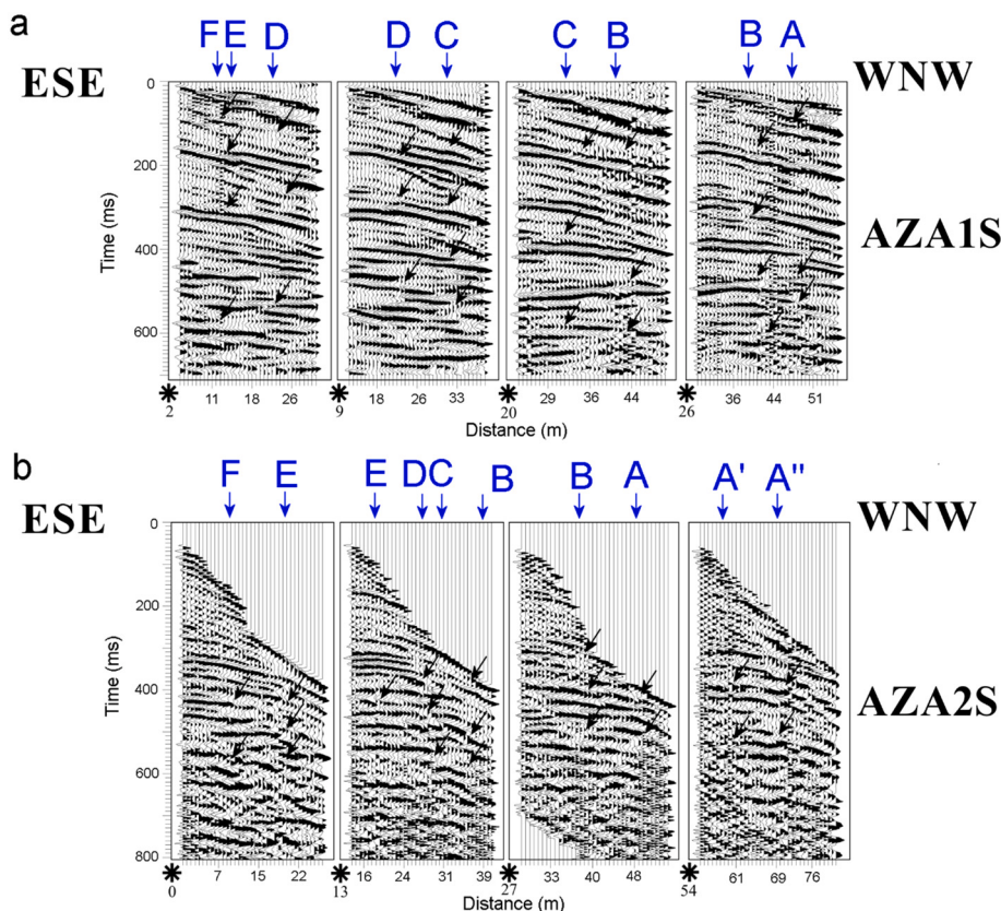
Fig. 8. (a) Raw field shot gathers from S-wave reflection profile 1 (AZA1S), with 10–100 Hz band-pass filtering. Undulations, amplitude changes, and breaks are apparent in reflection hyperbolae at locations which match with the locations of abrupt changes in velocity found in HOVA analysis (Fig. 9) and perturbations in the reflection events in the stacked sections (indicated by arrows). The letters in the top margin indicate the same locations as marked in stacked sections and HOVA panels shown in Figs. 5 to 7 and 9. (b) Same as (a) but for profile 2 (AZA2S); here the field shot gathers have been top-muted to remove direct wave and surface waves, to increase the visibility of the reflection events. The black stars with a number below indicate shot locations in meter.
