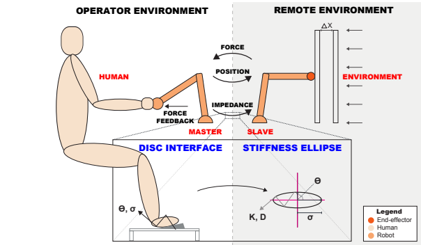
Fig. 1. Bilateral tele-impedance with the proposed foot-operated interface. The human operator controls the motion of the remote robot (slave) with a hand-operated haptic interface (master) and feels force feedback. The operator simultaneously controls the remote robot's stiffness ellipse through the disc interface using a foot. The shape of the stiffness ellipse is defined by orientation \theta and principal axes \sigma that determine how stiff the robot end-effector is in the respective direction of Cartesian space.
