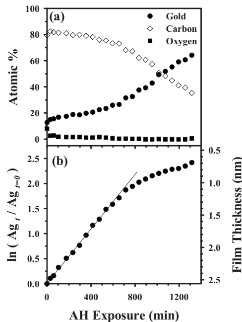
FIG. 4. (a) Changes in the elemental composition of a 2.6 nm thick electron beam deposited film, as a function of atomic hydrogen exposure ( P_{\text{H}_2} = 1.5 \times 10^{-5} Torr, \approx 4.9 \times 10^{15} H atoms \text{s}^{-1} \text{cm}^{-2} ). (b) The corresponding change in the film thickness during atomic hydrogen exposure has been determined by Eq. (1); a best-fit line has been fit through the region where the film thickness decreases linearly with atomic hydrogen exposure.
