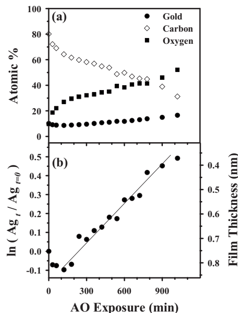
FIG. 7. (a) Changes in the elemental composition of a 0.76 nm thick gold, carbon, and oxygen film, formed by electron beam irradiation ( \approx 1.7 \times 10^{-4} \mu\text{W}/\mu\text{m}^2 , 30 min) of Au III (acac)Me 2 , as a function of atomic oxygen exposure ( P_{\text{O}_2} = 6.0 \times 10^{-7} Torr; \approx 2.0 \times 10^{14} O atoms \text{s}^{-1} \text{cm}^{-2} ). (b) The corresponding change in the film thickness during atomic oxygen exposure has been determined by Eq. (1); a best-fit line has been fit through the region where the film thickness decreases linearly with atomic oxygen exposure.
