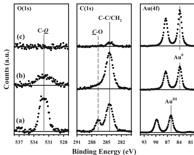
FIG. 3. XP spectra of the \text{Au}(4f) , \text{C}(1s) , and \text{O}(1s) regions of (a) a 2.8 nm thick molecularly adsorbed \text{Au}^{\text{III}}(\text{acac})\text{Me}_2 film on a silver substrate at \approx 160 K, (b) the same film after electron irradiation ( \approx 1.7 \times 10^{-4} \mu\text{W}/\mu\text{m}^2 , 30 min), and (c) the electron beam deposited film after 35 h exposure to atomic hydrogen ( P_{\text{H}_2} \approx 1 \times 10^{-5} Torr; \approx 3.3 \times 10^{15} H atoms \text{s}^{-1} \text{cm}^{-2} ).
