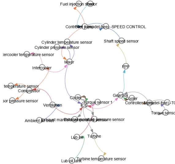
Fig. 4. Addition of hardware automation components in the knowledge graph. An excerpt of the semantic description of the additional hardware automation components can be found in Table II.
