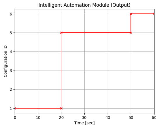
Fig. 6. Closed-loop configuration implementation by the intelligent automation module for the specified sensor fault scenario. The online switching mechanism is activated by the decisions of the monitoring agents regarding the occurrence of faults.
