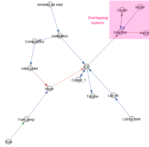
Fig. 3. Knowledge graph for diesel-electric propulsion. Each color of the edges represents a different medium used. The semantic description of the overlapping plant components (electrical propulsion cluster) shown in the shaded area is given in Table I
