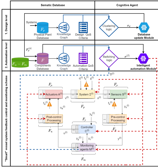
Fig. 2. Multi-level cognitive architecture for intelligent marine vessels. At the design level, the cognitive agent determines the system selection F_p^{(s)} from a physical plant database F_p of potential options based on design criteria. In the automation level, the cognitive agent determines the closed-loop configuration to be used based on the automation criteria and the monitoring agents decision D^{(I)} regarding the occurrence of faults ( f_a^{(I)} , f_p^{(I)} , f_s^{(I)} ).
