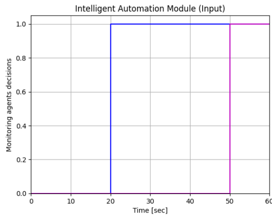
Fig. 5. Feedback of monitoring agents' decisions to the intelligent automation module for the specified sensor fault scenario (blue: monitoring agents' decision regarding the occurrence of faults in the shaft speed sensor, magenta: monitoring agents' decision regarding the occurrence of faults in the motor torque sensor). A value of '0' indicates that faults have not been diagnosed while a value of '1' indicates that faults were diagnosed.
