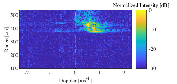
Fig. 2. Example of Range Doppler map for a walking motion, computed over a one second interval and with normalized intensity.
