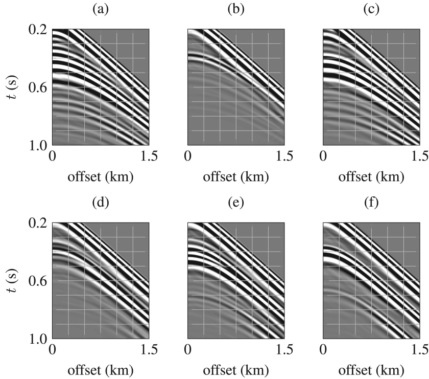
Figure 14. Modelled shot gathers at the last iteration corresponding to the multi-objective inversion in Figs 13. (a) After the first J_b inversion. (b) After the first J_{Is} inversion. (c) After the second J_b inversion. (d) After the second J_{Is} inversion. (e) After the third J_b inversion. (f) After the third J_{Is} inversion.
