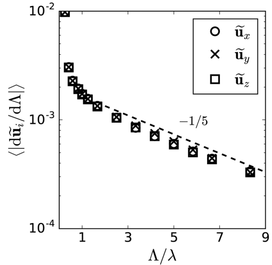
FIG. 16. Rate of change in the \tilde{\mathbf{u}}_i fields with an increase in \Lambda . Here, \langle \cdot \rangle denotes spatial averaging.
