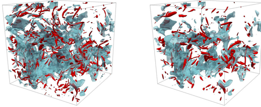
(a) Contours of E_k = 2\langle E_k \rangle (blue) along with \omega = 3\omega' (red) shows that these fields are spatially exclusive. (b) Contours of L = 2L' (blue) along with H^p = 5H^{p'} (red) shows that these correlation fields are spatially exclusive.
