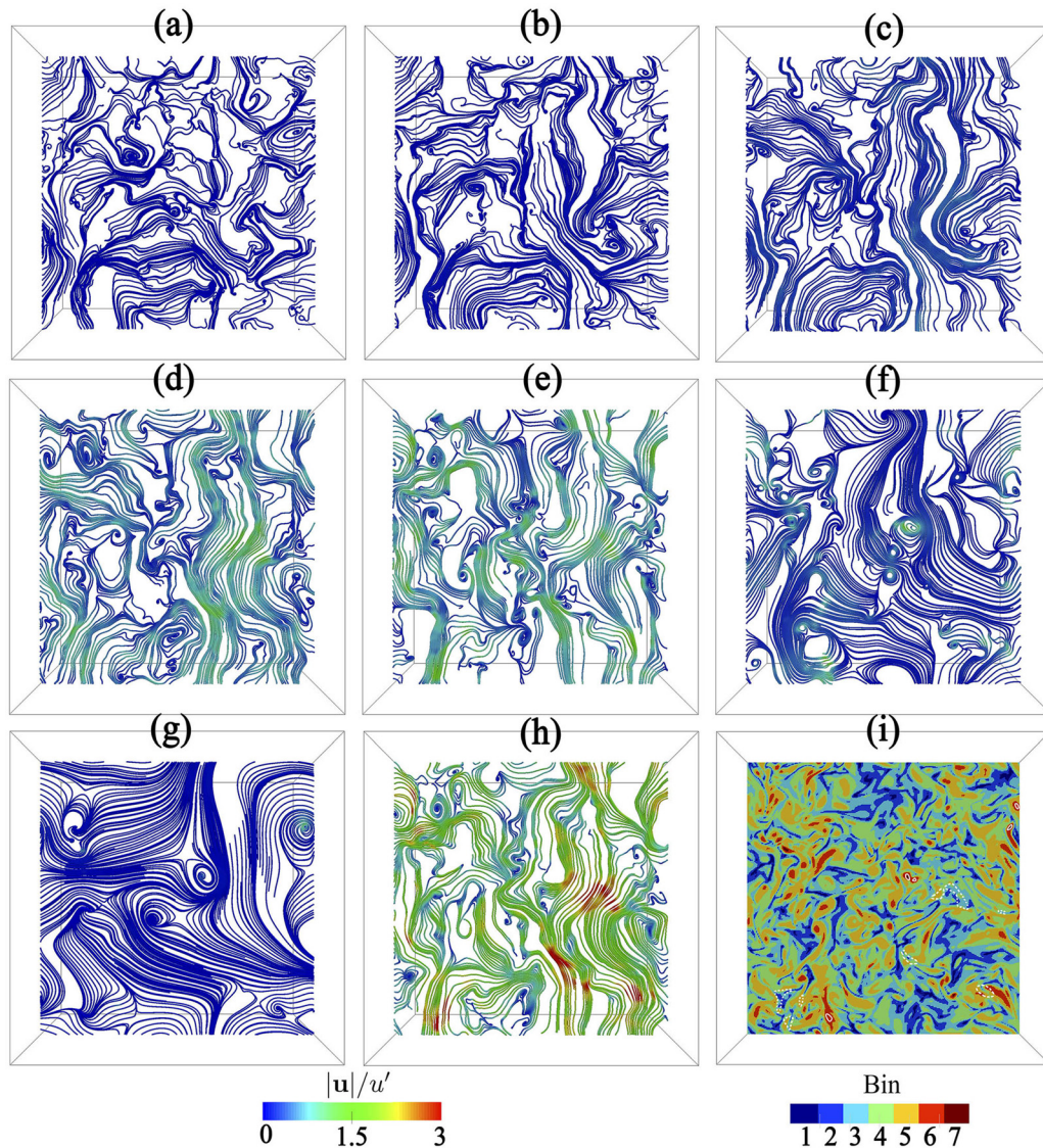
FIG. 24. Planar velocity streamlines (in the entire xy -plane, at an arbitrary z location) have been shown for Bin1 through Bin7 going from panels (a) through (g), while panel (h) shows the streamlines of the total velocity field. Panel (i) shows the vorticity field colored by the bin number, along with contours of 2.5L' (dashed white lines) and 5H^{p'} (solid white lines). Colorbar shows the velocity magnitude.
