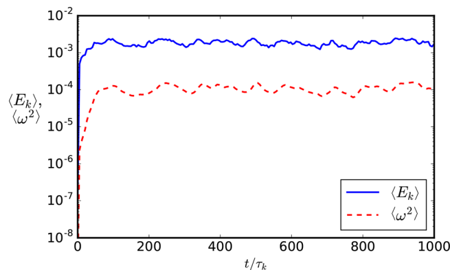
FIG. 10. Time evolution of the volume averaged turbulence kinetic energy \langle E_k \rangle and enstrophy \langle \omega^2 \rangle . Both quantities attain a steady-state value, reflecting a developed turbulence state.
