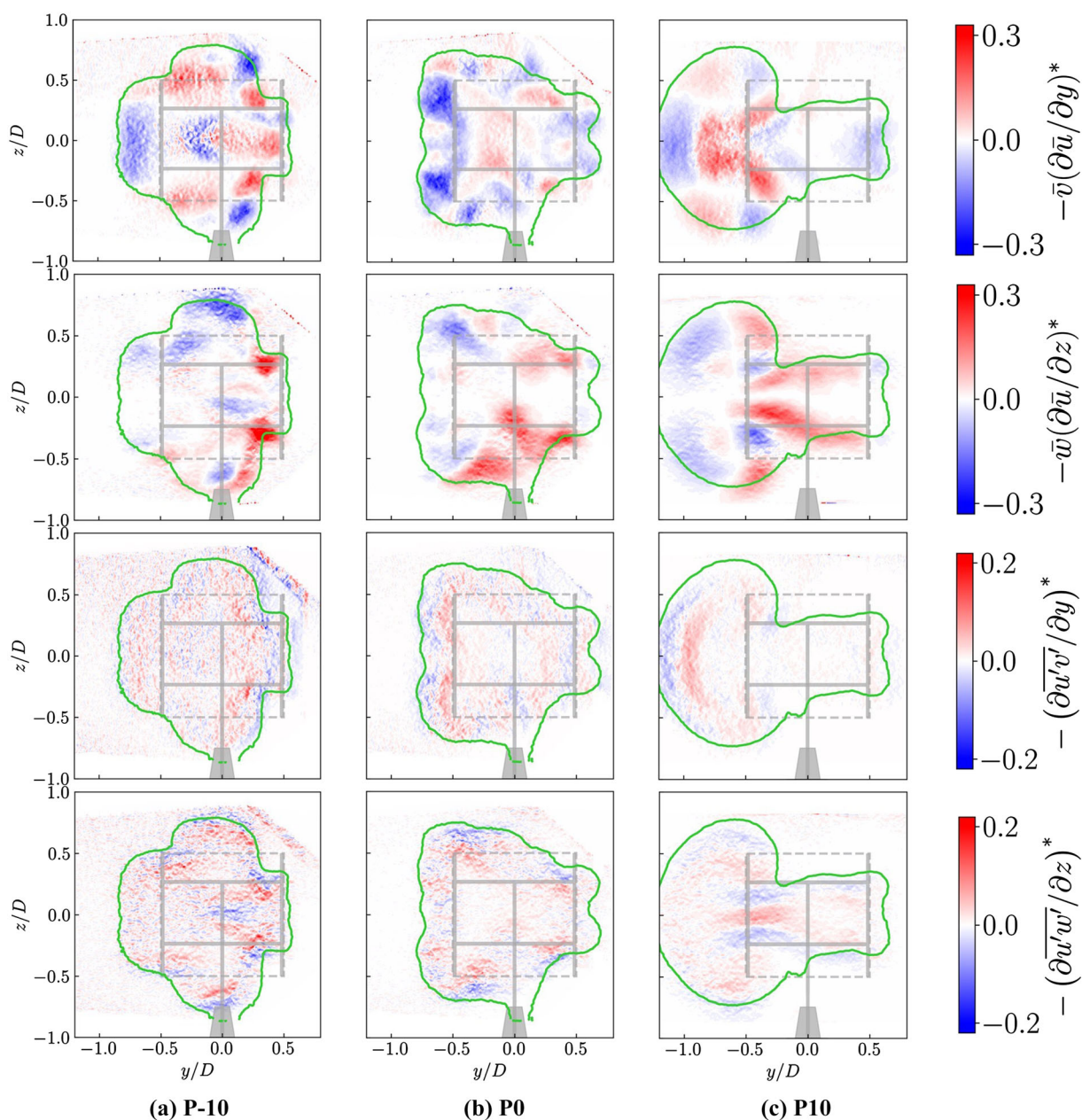
FIGURE 14 Measured terms of the RANS equation in the streamwise direction. For each case, the terms are normalized by the maximum value of \bar{u}(\partial \bar{u} / \partial x) , as denoted by * [Colour figure can be viewed at wileyonlinelibrary.com ]
