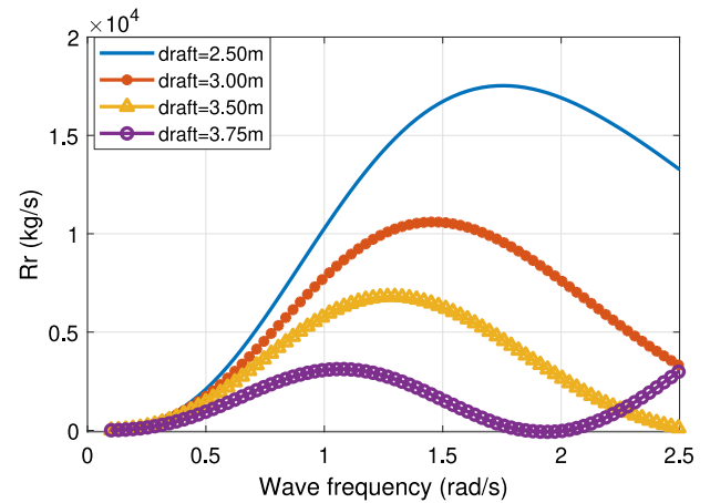
(c) Radiation damping
