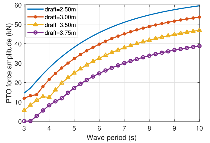
(a) PTO force amplitude (or maximum PTO force)
