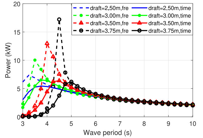
Fig. 12. Average power calculated by the nonlinear time domain model and frequency domain model for different buoy drafts. The results are calculated in regular wave states with a wave height of 1.0 m and the RMS of the PTO force limit is 10 kN. In the legend, “fre” and “time” represent the frequency domain model and nonlinear time domain model respectively.
