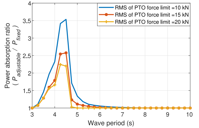
Fig. 10. Ratio of the power absorbed by the adjustable draft WEC to that by the fixed draft WEC in different RMS of the PTO force limit. The results are calculated in regular waves with a wave height of 1.0 m. P_{adjustable} and P_{fixed} embody the power absorbed by the adjustable draft WEC and the power absorbed by the WEC with a fixed draft of 2.5 m.
