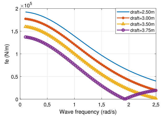
(a) Excitation force coefficients
