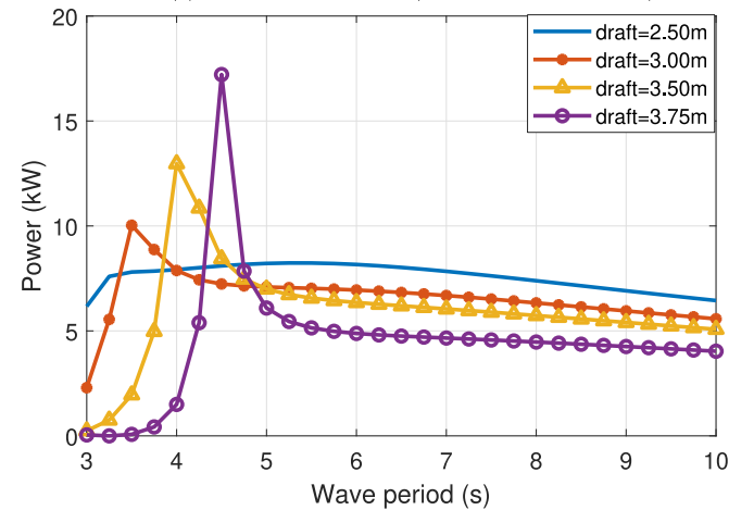
(b) PTO average power
