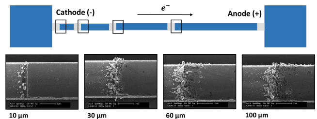
Figure 3.7. Test results for 10/30/60/100 μm Cu strips with TiN/Oxide/Cu structure under the current density of 1 MA/cm 2 at 250 °C.
