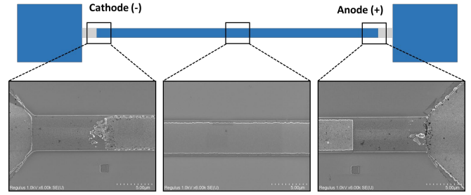
Figure 3.2. The test result of Cu stripes tested under the current density of 1 MA/cm 2 at 250 °C for 3 hours
