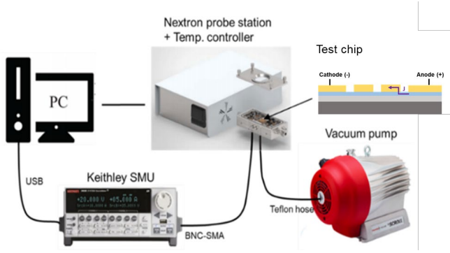
Figure 2.1. The schematic overview of the setup.
