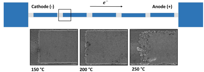
Figure 3.6. Test results for the sample containing 5 segments with the same length of 60 μm in TiN/Oxide/Cu system at different temperatures under the current density of 1 MA/cm 2 for 3 hours.
