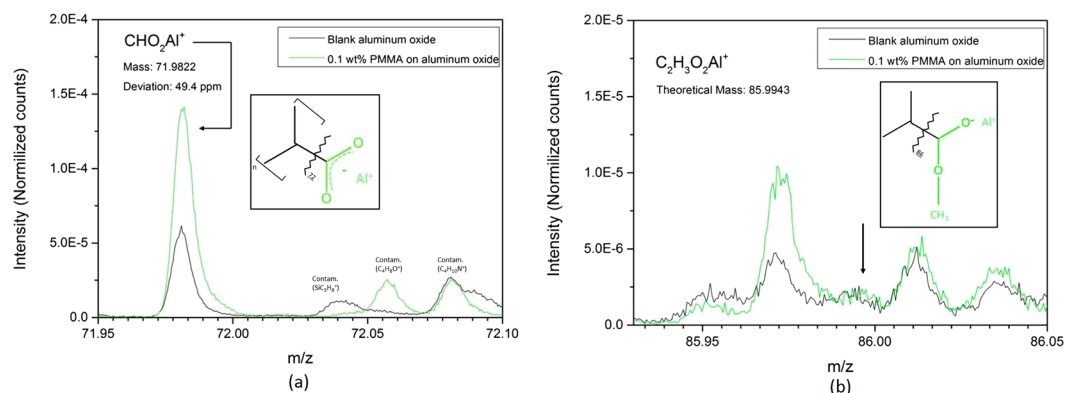
Figure 4. (a) ToF-SIMS spectra showing a fragment ( \text{CHO}_2\text{Al}^+ ) that indicates the carboxylate bond between PMMA and aluminum oxide showing that the polymer is ionically bonded to the metal oxide. (b) ToF-SIMS spectra showing the absence of a theoretical fragment ( \text{C}_2\text{H}_3\text{O}_2\text{Al}^+ ), that would be expected if the methoxy group of PMMA was present when the functional group is bonded to the interface. Insets: schematic representations of fragmentation of the monomer unit with ion fragment coloured in green. Mass is the experimentally obtained mass. The deviation (ppm) is the difference between the experimental and the theoretical mass.
