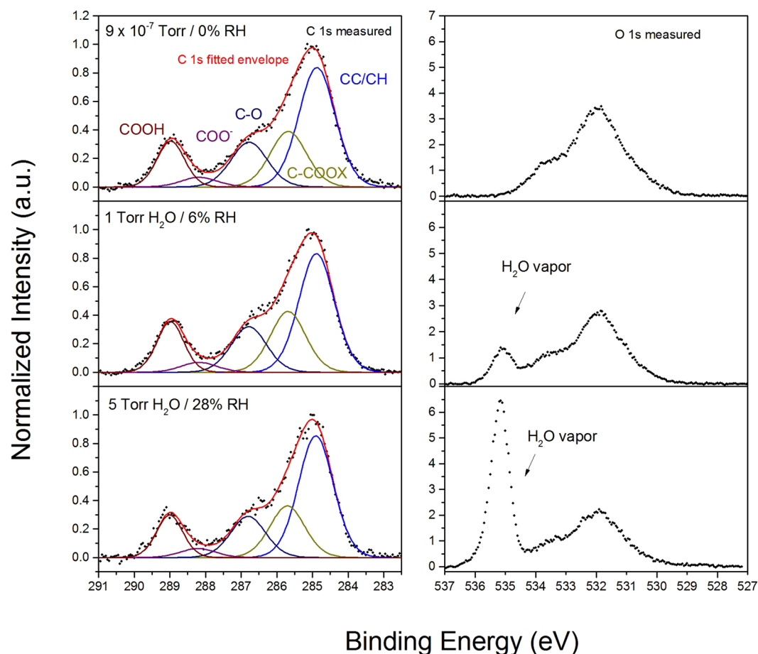
Figure 6. Normalized C 1s (left) and O 1s (right) APXPS spectra of an ultrathin PMMA film on native aluminum oxide at varying water vapor pressures. 9 \times 10^{-7} Torr (a), 1 Torr \text{H}_2\text{O} (b), 5 Torr \text{H}_2\text{O} (c).
