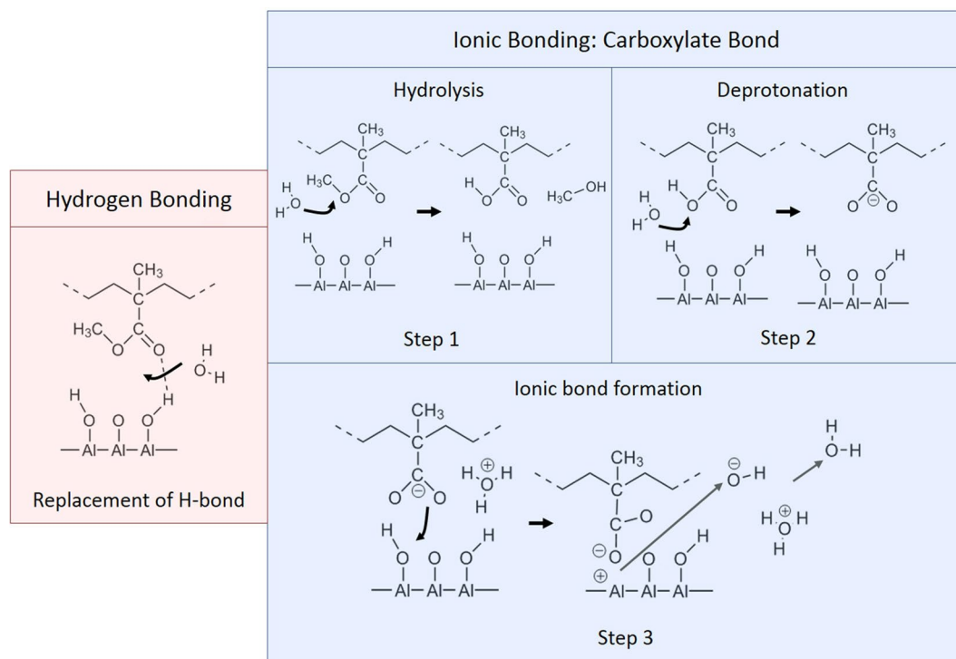
Figure 7. Schematic representation of the adsorption mechanism of PMMA on native aluminum oxyhydroxide and the effect of water on the formed bonds. Hydrogen bonds between the carbonyl group of PMMA and the surface hydroxyl groups are replaced by water. The carboxylate ionic bond formation is enabled/enhanced by water molecules at the interface. First a hydrolysis of the methoxy group takes place forming methanol (Step 1). Then the carboxylic acid group is deprotonated to form a carboxylate anion (Step 2), which reacts with a free surface hydroxyl group resulting in an ionic bond at the interface (Step 3). In this schematic representation, the coordination type of the ionic bond is not taken into account.
