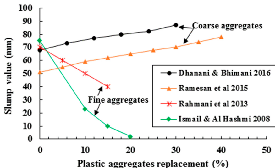
Figure 3. Influence of coarse and fine plastic aggregates on the concrete slump.
