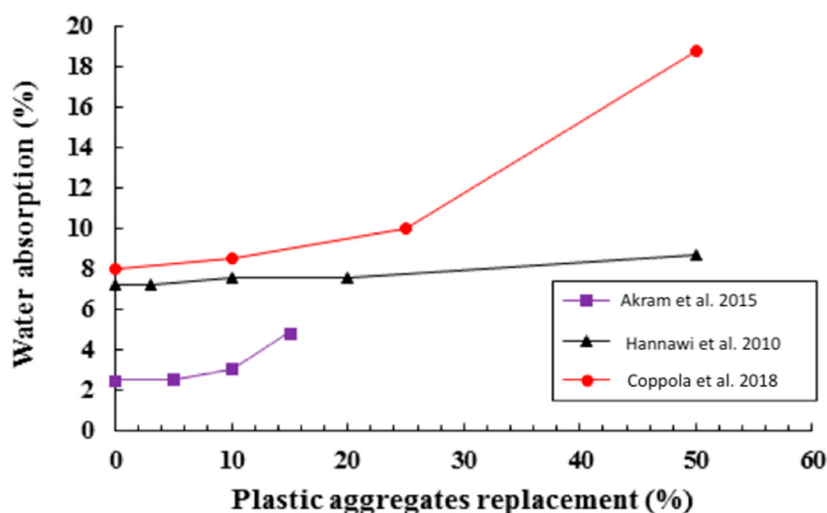
Figure 15. Water absorption capacity of concrete with plastic aggregates.
