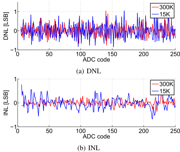
Fig. 13. Non-linearities (DNL and INL) extracted from ADC density test. The ADC density is produced by applying a ramp that exceeds both negative and positive input range to the input of the ADC.
