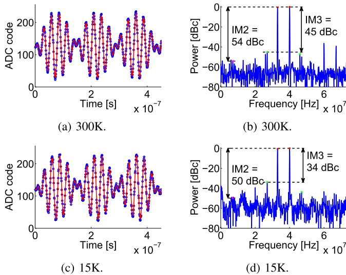
Fig. 19. IM2 and IM3 derived with a two tone test at 33 and 40 MHz.
