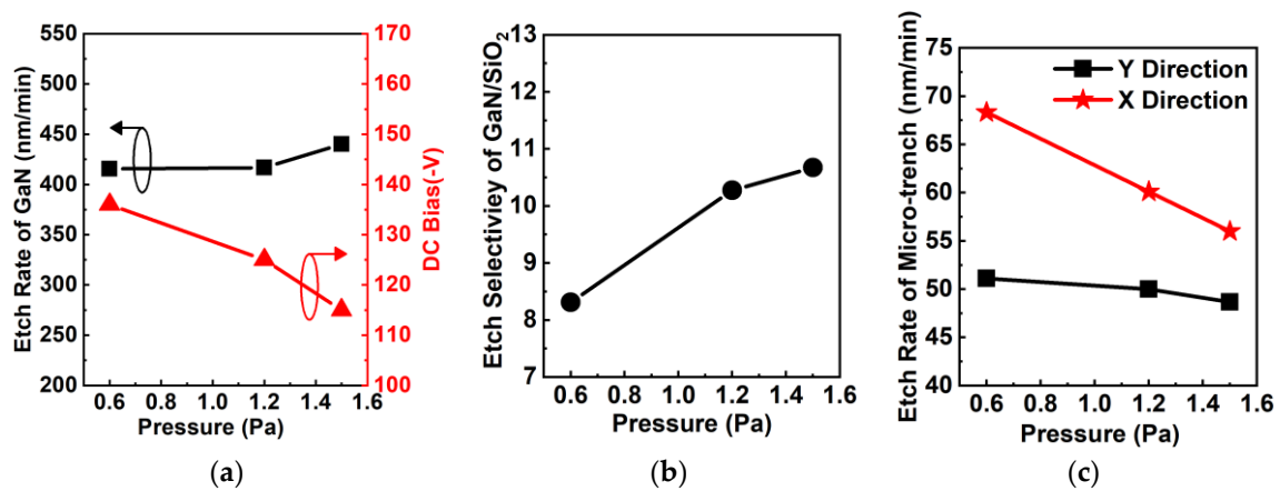
Figure 11. (a) Etching rate of GaN and DC bias as a function of pressure. (b) Etching selectivity of GaN over \text{SiO}_2 as a function of pressure. (c) The effect of pressure on etching rates of the microtrench in the X and Y directions.
