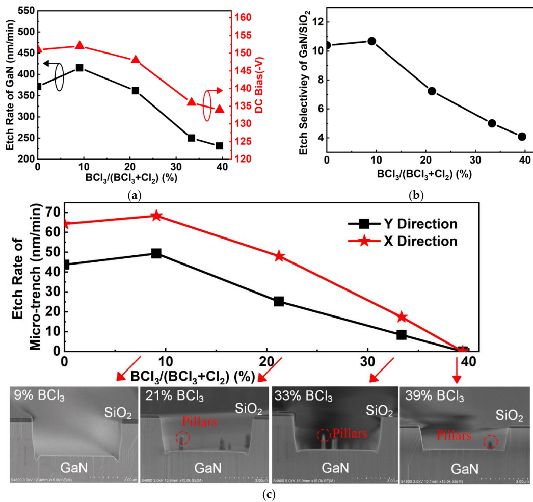
Figure 10. (a) Etching rate of GaN and DC bias as a function of \text{BCl}_3 content in the \text{Cl}_2/\text{BCl}_3 gas mixture. (b) Etching selectivity of GaN over \text{SiO}_2 as a function of \text{BCl}_3 content in the \text{Cl}_2/\text{BCl}_3 gas mixture. (c) The effect of \text{BCl}_3 content in the \text{Cl}_2/\text{BCl}_3 gas mixture on etching rates of the microtrench in the X and Y directions. The insets of (c) show cross SEM images for samples etched with different \text{BCl}_3 concentrations.
