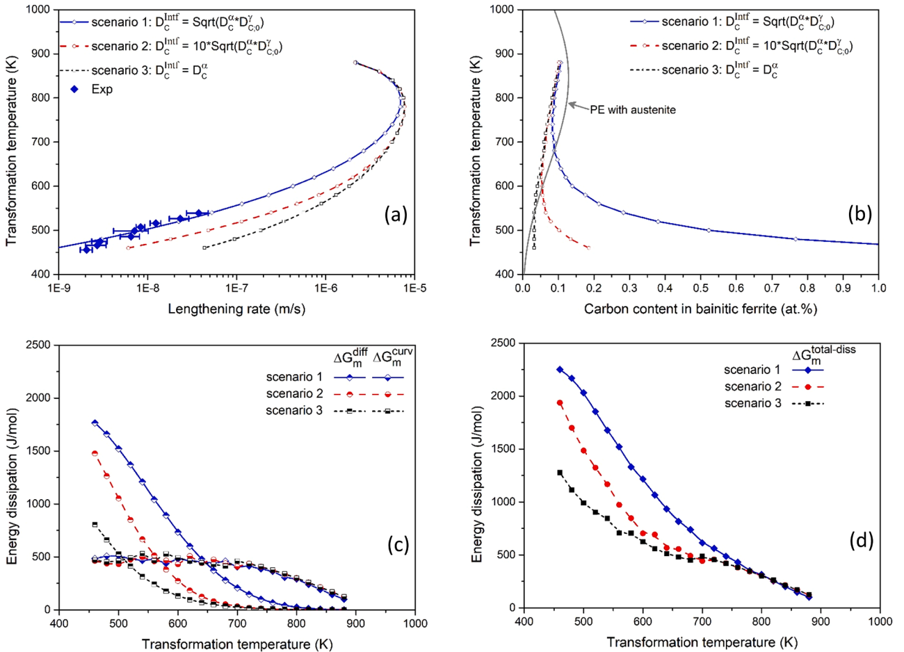
Fig. 11. The predicted (a) lengthening rates and (b) carbon content in bainitic ferrite for the HC-2 steels in three scenarios with different D_C^{\text{Intf}} . (c) \Delta G_m^{\text{curv}} , \Delta G_m^{\text{diff}} and (d) \Delta G_m^{\text{total-diss}} as a function of transformation temperature for three scenarios.
