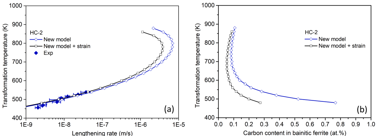
Fig. 12. The (a) lengthening rates and (b) carbon content in bainitic ferrite for the HC-2 steels predicted with and without considering the transformation strain.
