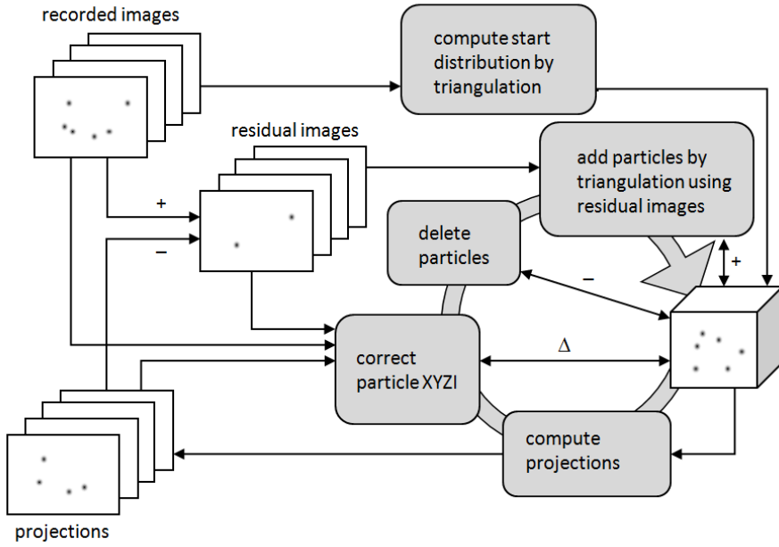
Figure 7.1. Flow chart of iterative particle reconstruction method.
