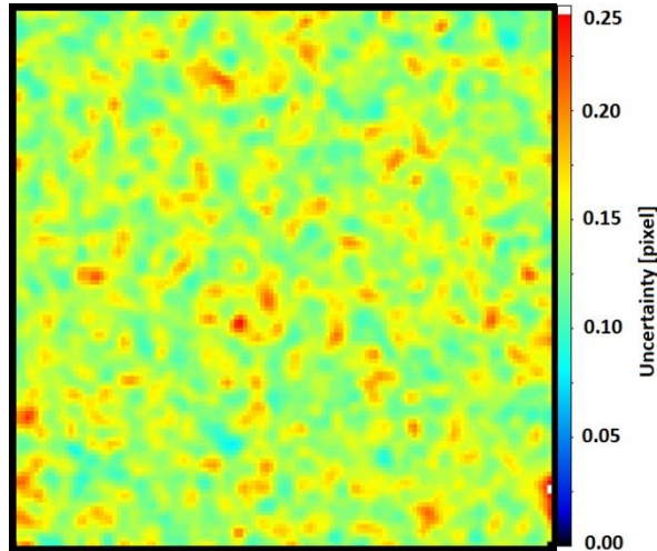
Figure 3.16. Typical uncertainty field with an average of 0.142 px and stdev of 0.018 px.
