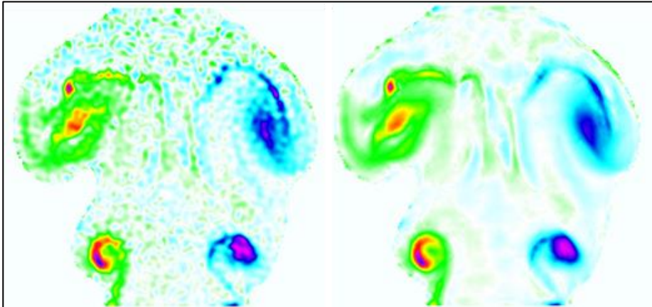
Figure 5.11. Ring vortex processed with 24x24 windows and 75% overlap without (left) and with denoising (right, S=3.5 ). Seeding and PIV processing is only applied inside the vortex. Color = vorticity (a.u.).
