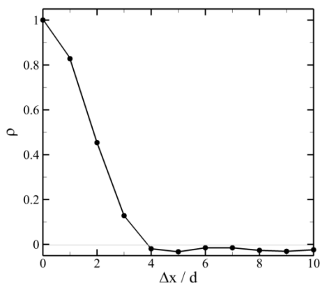
Figure 4.2. Spatial auto-correlation of the measurement error for interrogation window of 32 \times 32 pixels and 75% overlap (see also Figure 2.7, Figure 2.12, and Figure 2.13).
