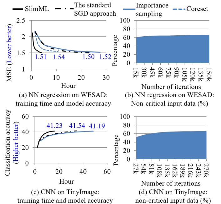
Fig. 11. Comparison of training time and accuracy with baseline techniques
