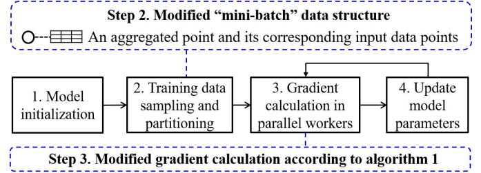
Fig. 7. The Distributed optimizer function in MLLib/BigDL
