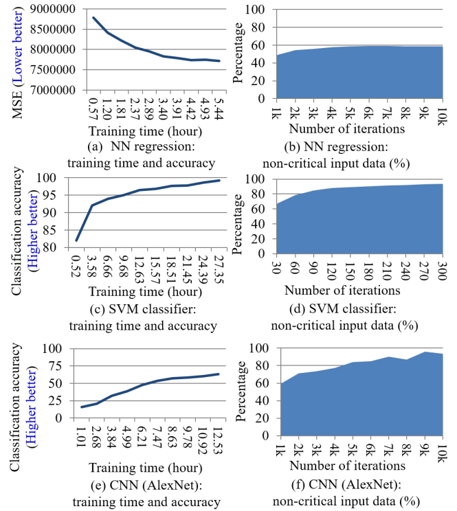
Fig. 3. Quantitative measurement of NN regression, SVM, and CNN
