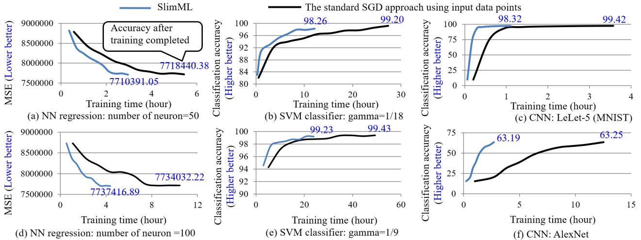
Fig. 10. Comparison of training time and accuracy with and without removal of non-critical input data in standard SGD approach
