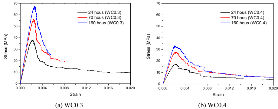
Fig. B.1. Simulated stress-strain curves of cement pastes under a tensile load.
