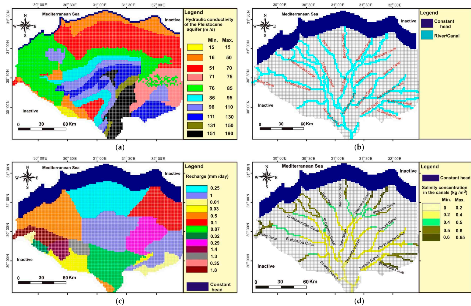
Figure 3. (a) The hydraulic conductivity of the Pleistocene aquifer of the Nile Delta. (b) Irrigation network. (c) Zones with different recharge rates in the Nile Delta. (d) The salinity concentration in kg/m 3 the river package, modified from data used in [5].
