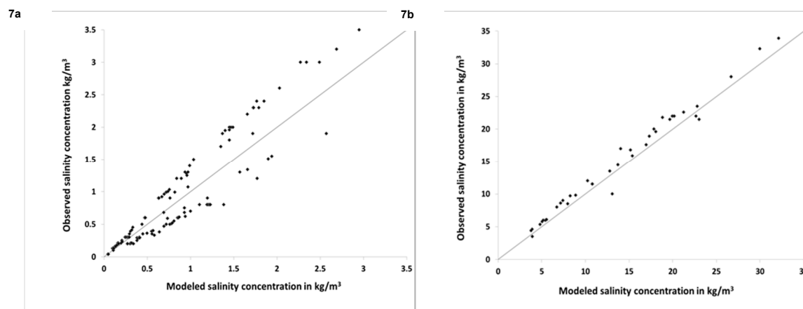
Figure 7. Modeled versus observed salinity concentrations in: (a) The southern and the middle parts of the NDA (RMSE = 0.8, Abs. Diff. = 0.52, Stan Dev. = 0.61 \text{kg}/\text{m}^3 ). (b) The northern parts of the NDA year 2010 (RMSE = 0.2, Abs. Diff. = 0.14, Stan Dev. = 0.11 \text{kg}/\text{m}^3 ).
