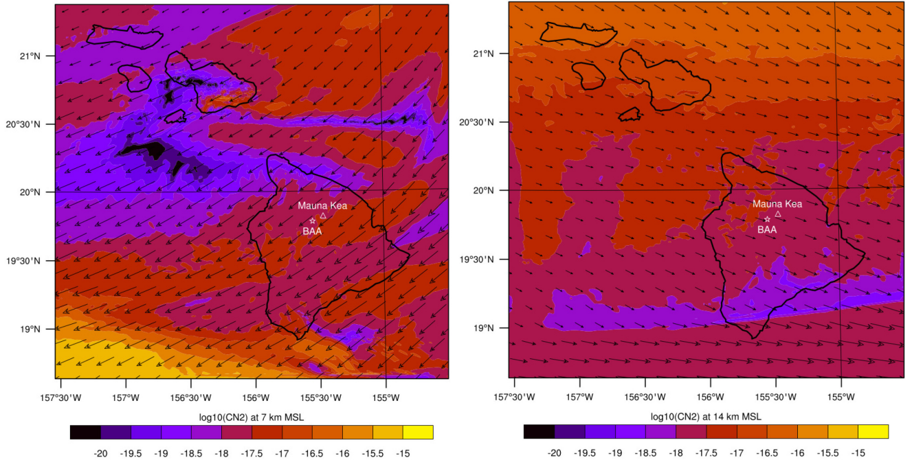
Figure 7. Contour plots of C_n^2 at the height of 7 km (left-hand panel) and 14 km (right-hand panel) above MSL. The overlaid arrows denote the velocity vectors at that height. The simulated data is from R_4 run and corresponds to 5 UTC of 2002 December 12. The thermosonde launch site and the Mauna Kea summit are demarcated by a white star and a white triangle, respectively.
