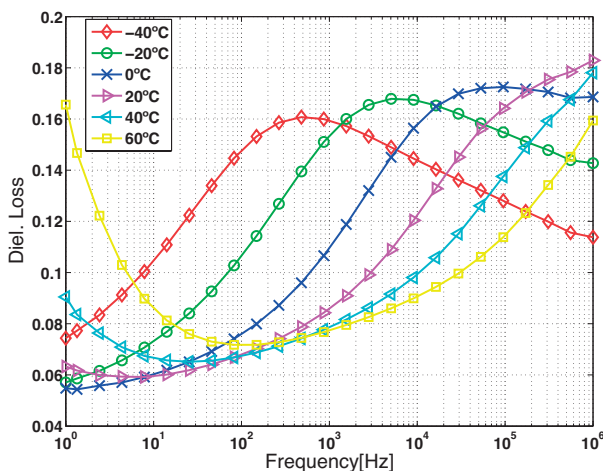
Figure 5.3: Dielectric losses of EP-I material samples as a function of frequency at temperatures between -40 °C and 60 °C. The frequency range is 1 Hz to 1 MHz.
