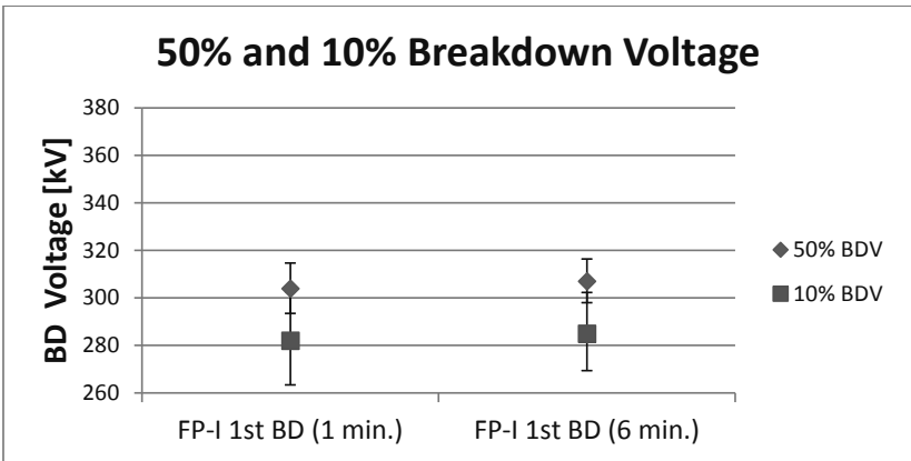
Figure 4.13: Comparison of 50% and 10% 1st Breakdown voltage of FP-I coated electrodes including 95% confidence intervals regarding addition of test results with 6 minutes waiting time between impulses.
