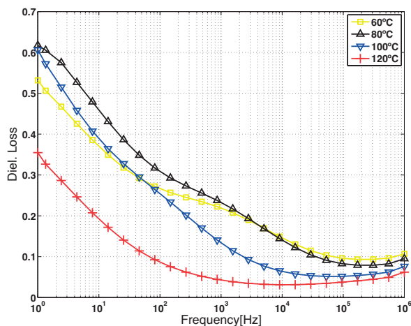
Figure 5.13: Dielectric losses of FP-IV material samples as a function of frequency at temperatures between 60 °C and 120 °C.
