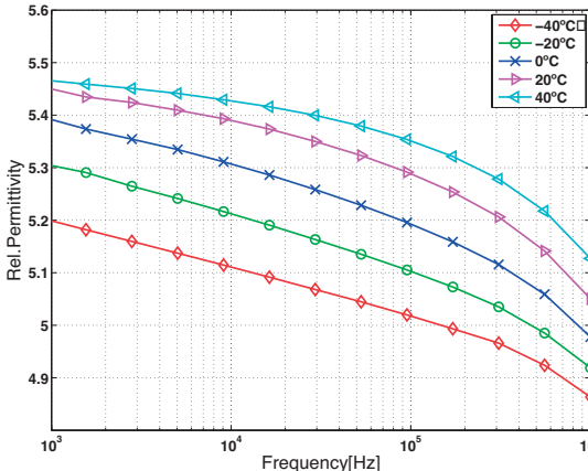
Figure 5.24: Relative permittivity of FP-II material samples as a function of frequency at temperatures between -40 °C and 40 °C. The frequency range is 1 kHz to 1 MHz.
