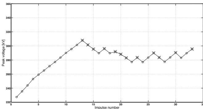
Figure 3.31: Combined test with step-up to breakdown and 50% up-down (the circles represent impulse applications and the crosses represent disruptive discharges).
