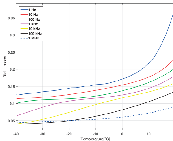
Figure 5.21: Detail of the dielectric losses as a function of temperature for frequencies between 1 Hz and 1 MHz. The temperature range is -40°C and 20°C.
