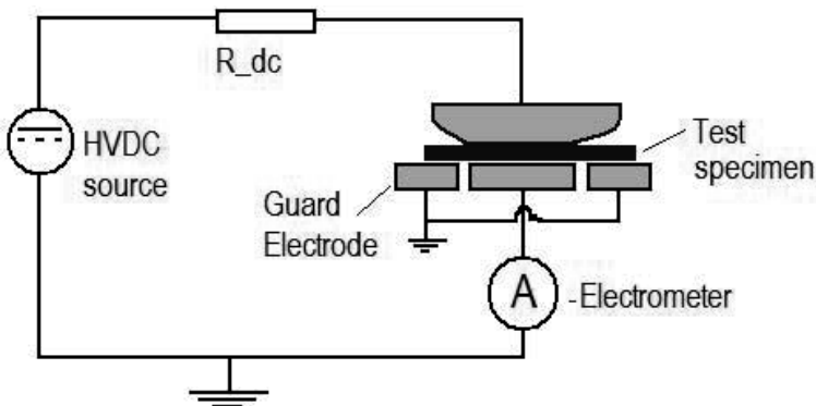
Figure 3.35: Schematic drawing of the conduction current setup.
