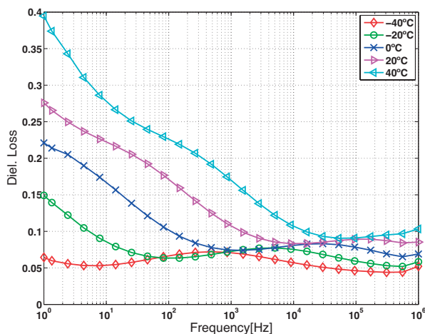
Figure 5.12: Dielectric losses of FP-IV material samples as a function of frequency at temperatures between -40°C and 40°C. The frequency range is 1 Hz to 1 MHz.
