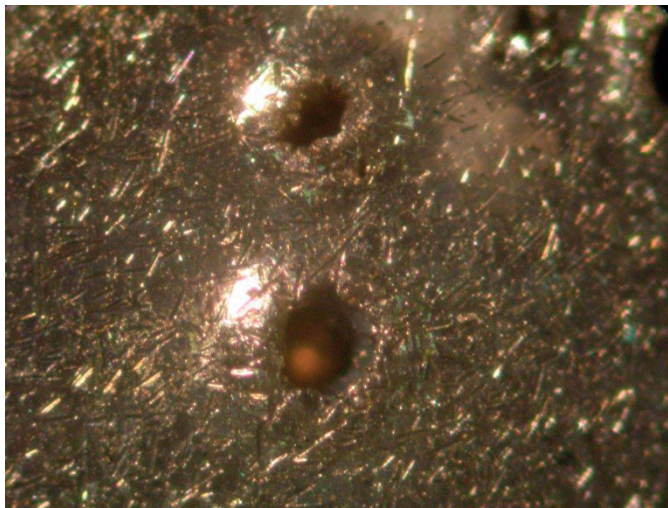
Figure 5.43: Microscopic view of the surface of a double layer FP-II – FP-I coated electrode after a breakdown test.
