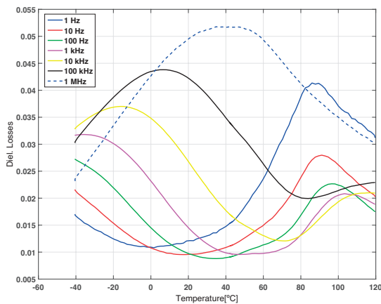
Figure 5.9: Dielectric losses of FP-I material samples as a function of temperature for frequencies between 1 Hz and 1 MHz. The temperature range is -40 °C to 120 °C.
