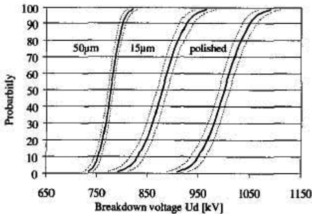
Figure 2.11: Normal distribution of breakdown voltage including 95% confidence intervals, positive LI voltage, s = 40 mm, variation of R_z , uncoated [10]
