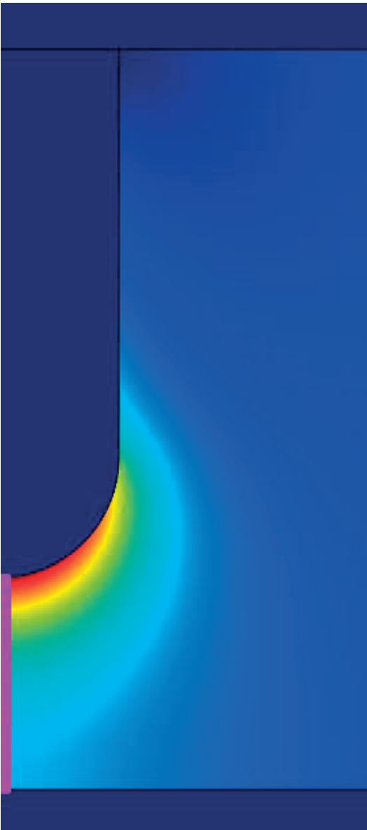
Figure 6.2: 2D rotational symmetric electric field calculation in rod-plane gap. The purple line represents the evaluation line.
