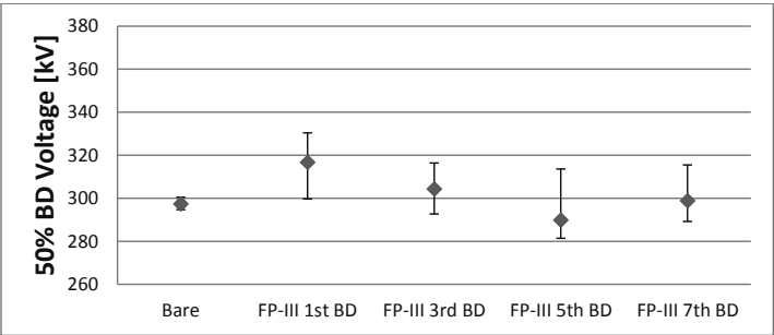
Figure 4.22: 50% Breakdown voltage of FP-III coated electrodes including 95% confidence intervals.
