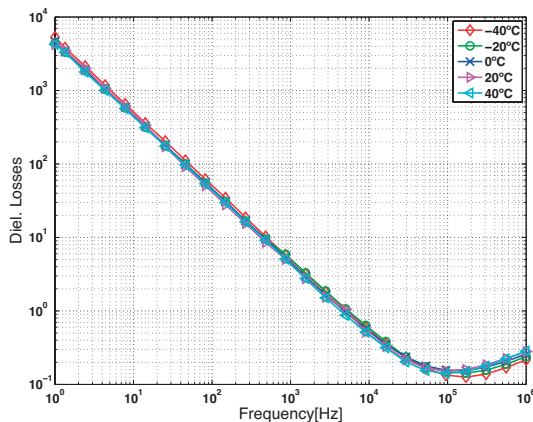
Figure 5.23: Dielectric losses of FP-II material samples as a function of frequency at temperatures between -40 °C and 40 °C. The frequency range is 1 Hz to 1 MHz.
