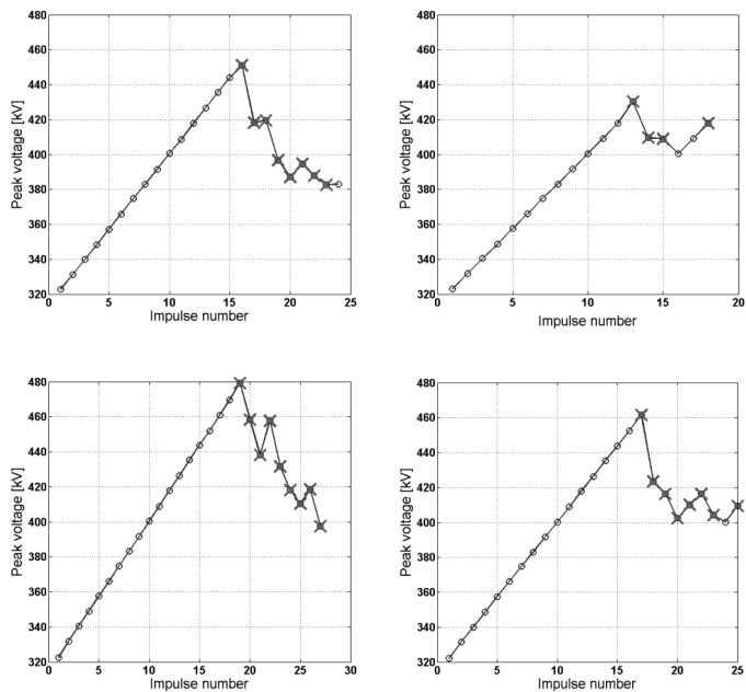
Figure A.26: Large size PA11 – Top left: series 5, batch 3, electrode 1, Top right: series 5, batch 3, electrode 2, Bottom left: series 5, batch 3, electrode 3, Bottom right: series 5, batch 3, electrode 4
