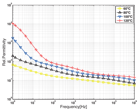
Figure 5.17: Relative permittivity of PA11 material samples as a function of frequency at temperatures between 60 °C and 120 °C. The frequency range is 1 Hz to 1 MHz.
