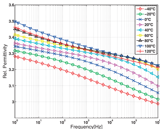
Figure 5.5: Relative permittivity of FP-I material samples as a function of frequency at temperatures between -40°C and 120°C. The frequency range is 1 Hz to 1 MHz.
