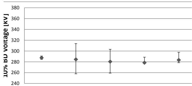
Figure 4.23: 10% Breakdown voltage of FP-III coated electrodes including 95% confidence intervals.
