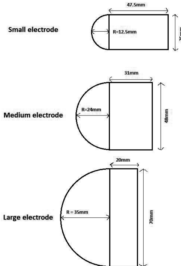
Figure 3.5: Dimensions of the three rod electrode types.
