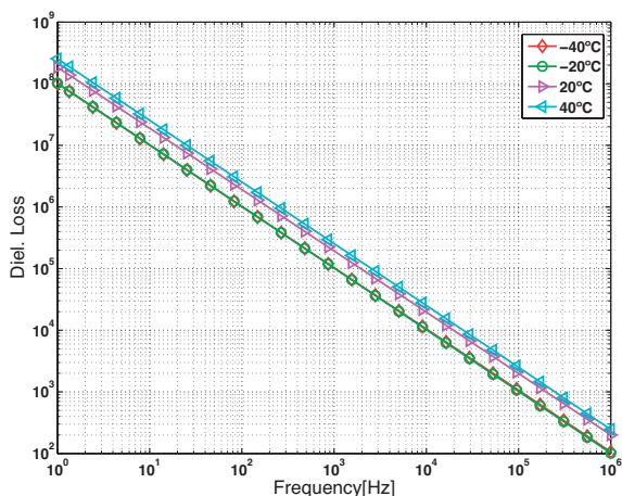
Figure 5.22: Dielectric losses of FP-III material samples as a function of frequency at temperatures between -40 °C and 40°C. The frequency range is 1 Hz to 1 MHz.
