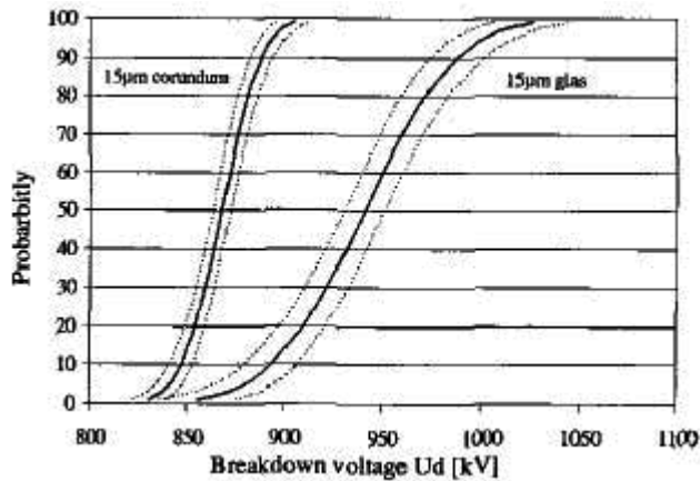
Figure 2.13: Normal distribution of breakdown voltage including 95% confidence intervals, negative LI voltage, s = 50 mm, R_z = 15 \mu\text{m} , varying surface treatment, uncoated [10]
