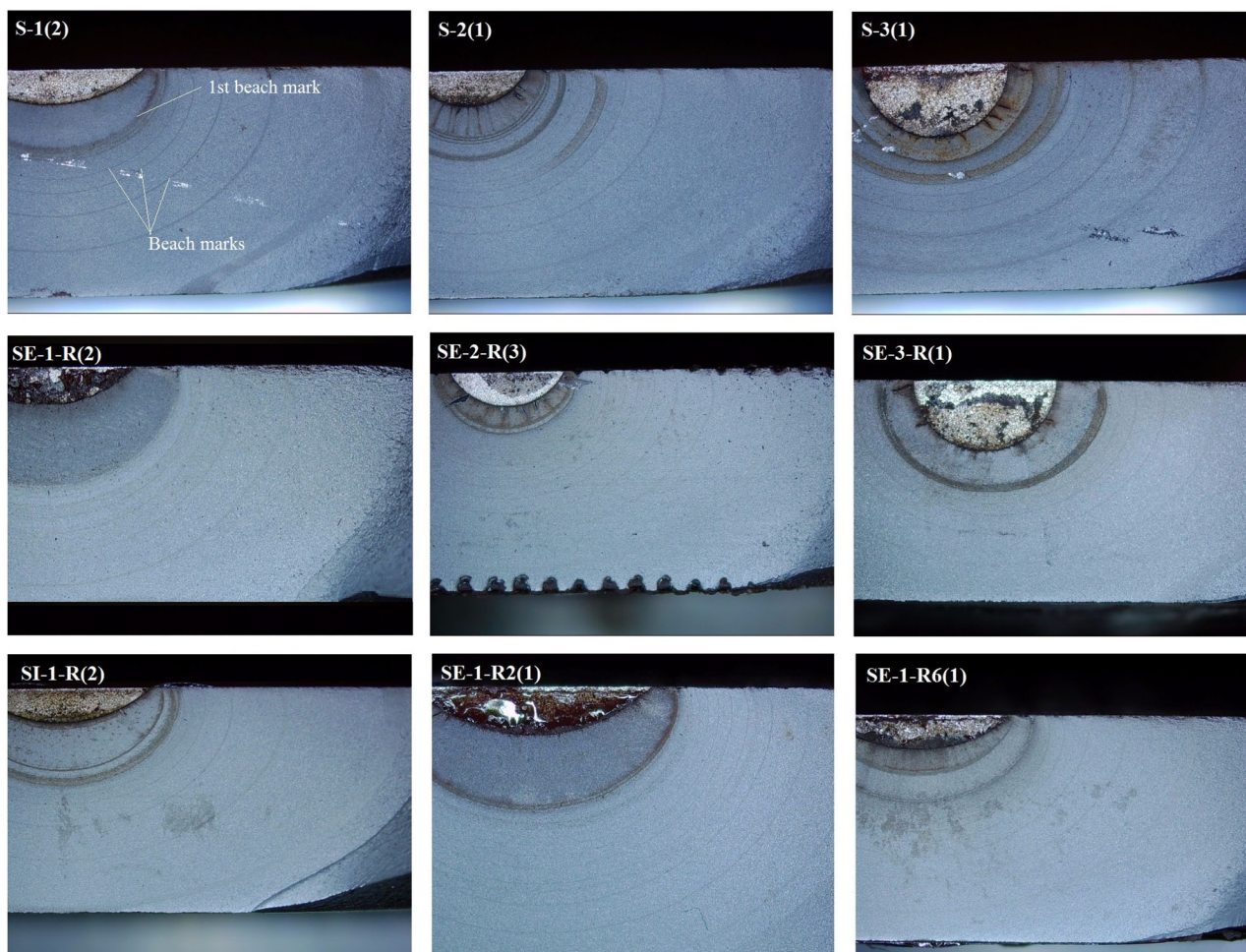
Figure 10. Beach marks on the cross-section of the steel plate specimens.
