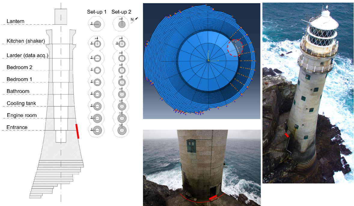
Fig. 3. Fastnet Lighthouse: (left) vertical section through structure and accelerometer arrangements in two sets, (mid upper) FEM showing door, (mid lower) view of rock restraint from stump of old tower, (right) drone view showing extended courses. Measurement x axis is through door, FEM x axis is rotated 22.5^\circ clockwise from door. Photos: James Bassitt and Athanasios Pappas.
