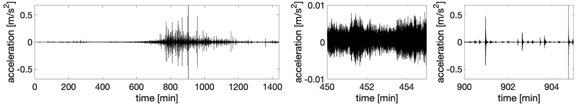
Fig. 13. Wolf Rock acceleration response during ex-Hurricane Ophelia, 16th October 2017. Left, for the whole day, middle for 7.30 AM (low tide), right for 3 PM.
