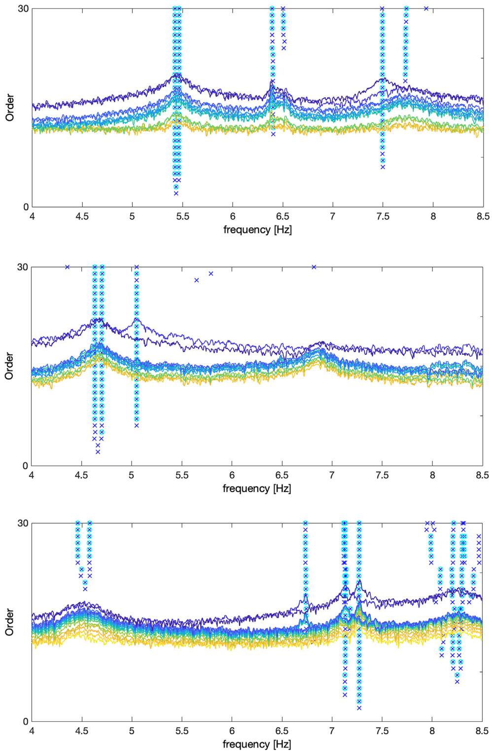
Fig. 7. SSI-COV applied to Les Hanois (upper), Wolf Rock (middle) and Eddystone (lower) data.
