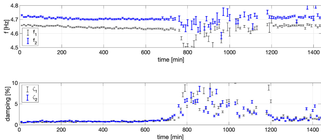
Fig. 16. Wolf Rock monitoring. Frequency estimation (upper) and damping estimation (lower) from application of BAYOMA to data of Fig. 16.
