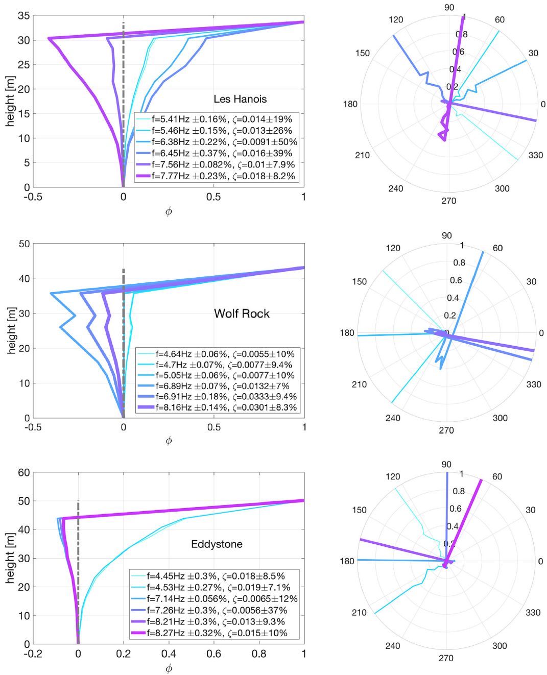
Fig. 8. BAYOMA modes. Left elevation, rotated to same plane; right in plan.
