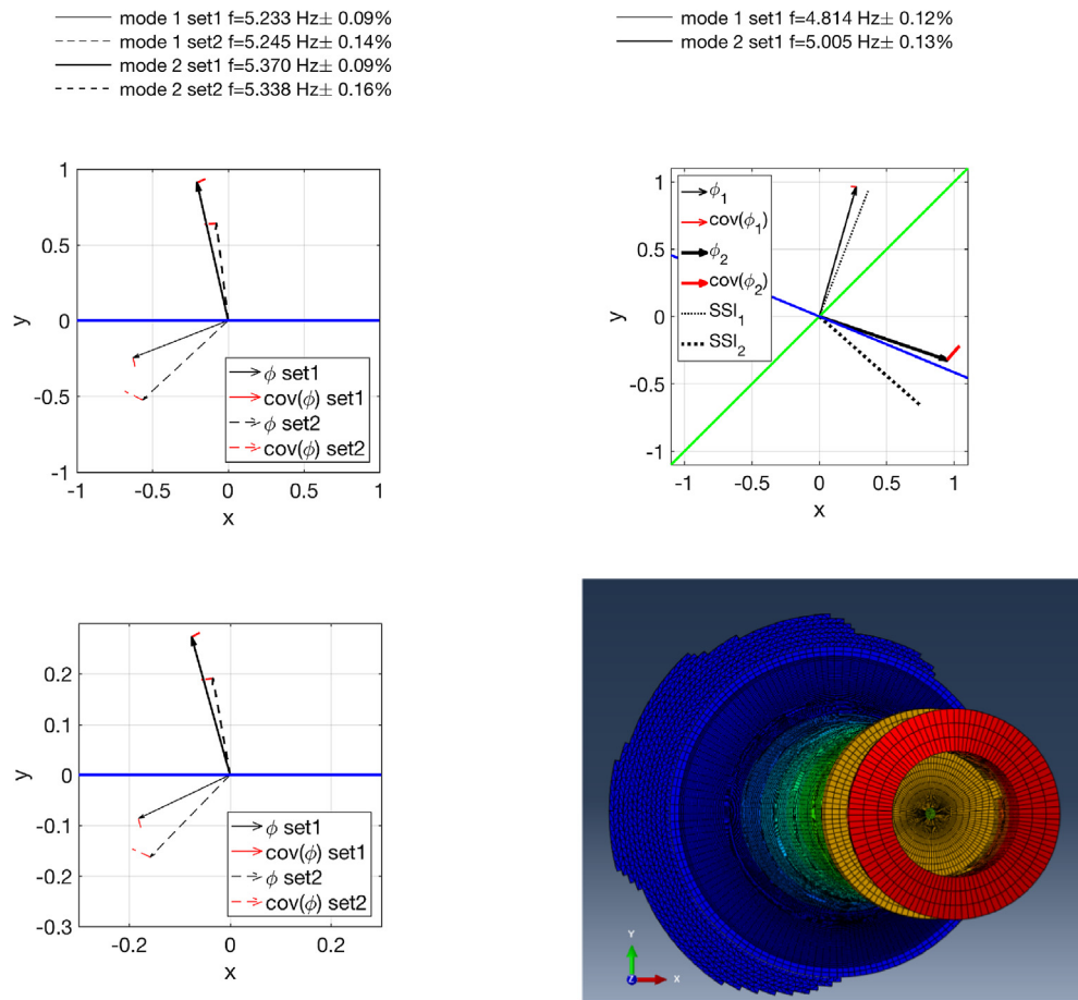
Fig. 11. Left column Dubh Artach level 7 (upper) and level 3 (lower); x axis (blue line) is aligned with openings (windows, doors). Right column Fastnet; x axis aligns with entrance, green line is North-South axis, blue line is x axis of FEM. FEM second mode, along the model axes shown bottom right. (For interpretation of the references to colour in this figure legend, the reader is referred to the web version of this article.)
