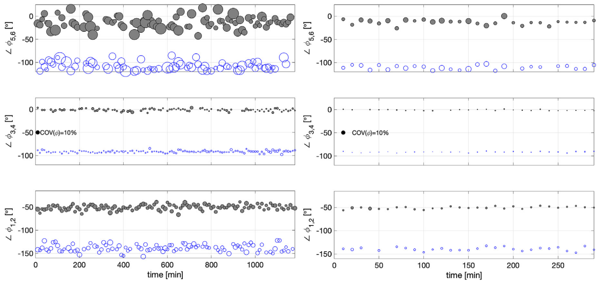
Fig. 15. Mode shape variation for (bottom to top) first, second and third mode shape pairs corresponding to Fig. 14. Size of circles reflects 1\sigma identification uncertainty on individual estimate.
