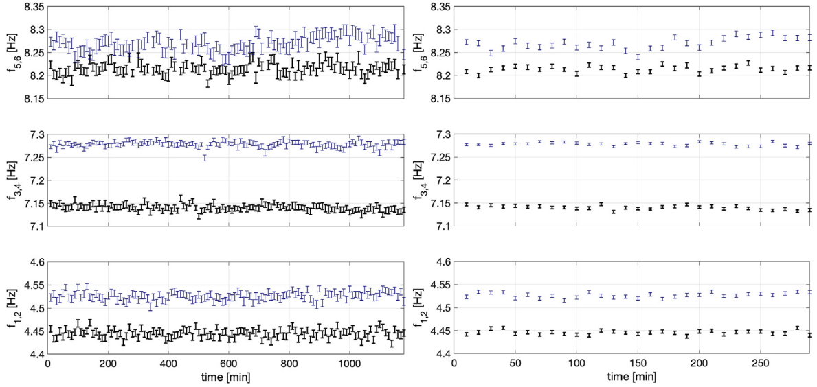
Fig. 14. Mode pair frequency variation for overnight recording at Eddystone Lighthouse.
