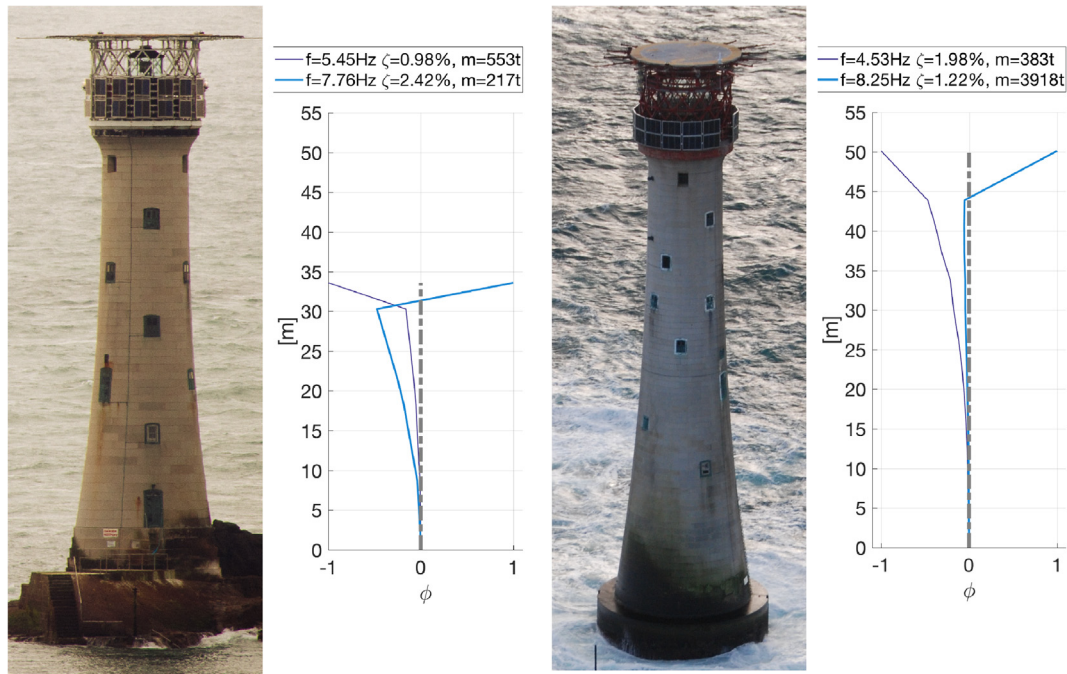
Fig. 1. Les Hanois (left) and Eddystone (right) Lighthouses and first two modes identified from experimental modal analysis of forced vibration test data for nominal x direction. Photos: Emma Hudson (left), Trinity House (right).
