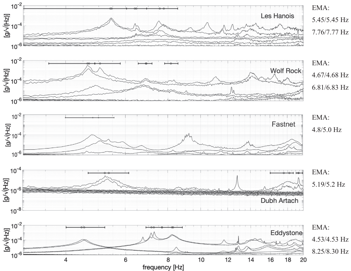
Fig. 6. Singular value decomposition of averaged ambient response data spectra, with corresponding mode frequencies identified by experimental modal analysis (EMA) of shaker test data with arbitrary orthogonal axes. Error bars indicate frequency bands manually chosen for BAYOMA identification and circles indicate BAYOMA-identified mode frequency (most probable values).
