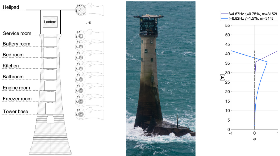
Fig. 2. Wolf Rock Lighthouse. Vertical section through tower, accelerometer angles; aerial view of lighthouse and landing area; EMA modes. Photo: James Bassitt.
