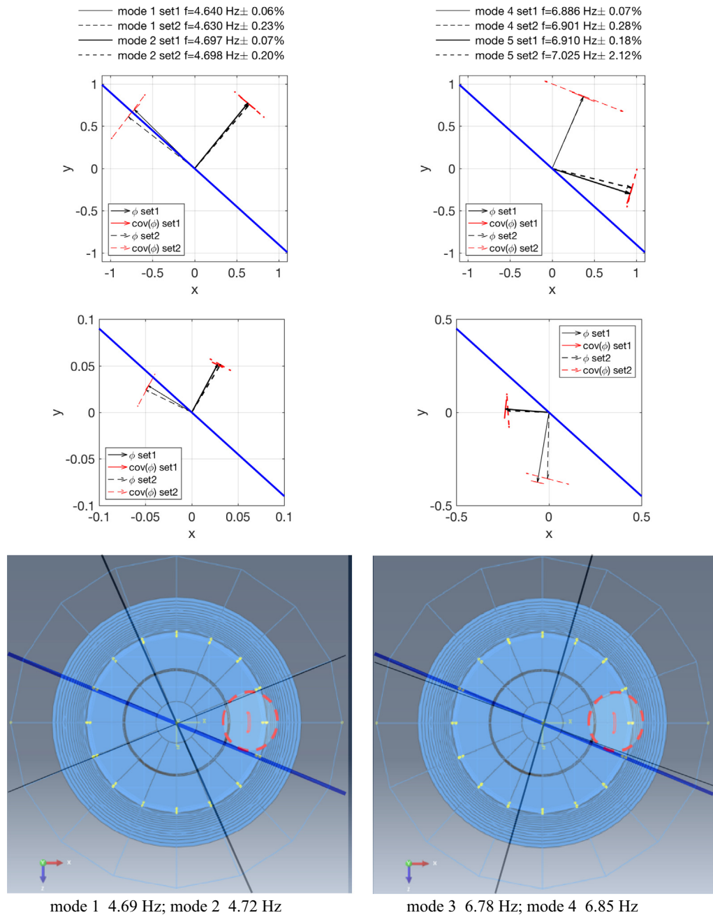
Fig. 10. Wolf Rock first (left columns) and second (right columns) mode pairs. Level 9 (upper) and 8 (middle). FEM modes (lower), red curve locates upper door. (Thick) blue lines are in direction of landing platform (also the entrance). (For interpretation of the references to colour in this figure legend, the reader is referred to the web version of this article.)
