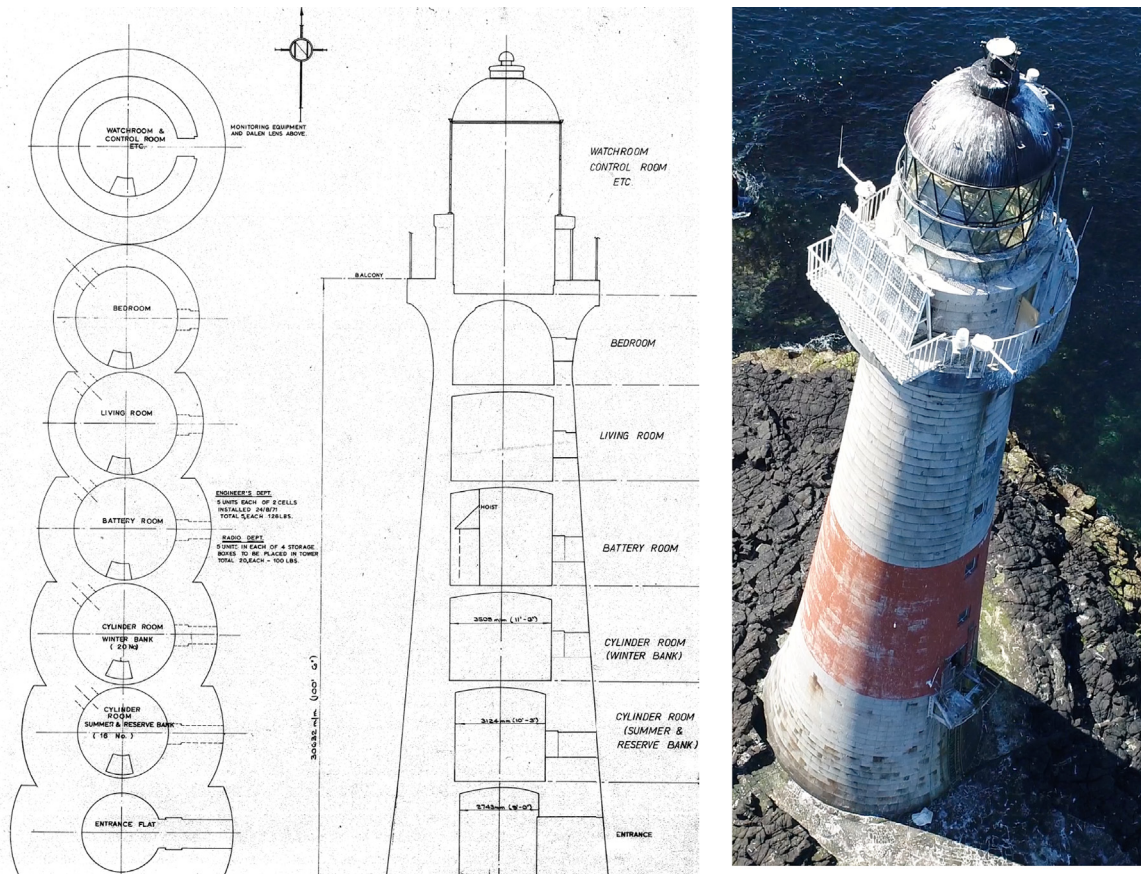
Fig. 4. Dubh Artach Lighthouse horizontal and vertical sections and aerial view, showing alignment of openings. Photo: James Bassitt, drawings courtesy of Trinity House.
