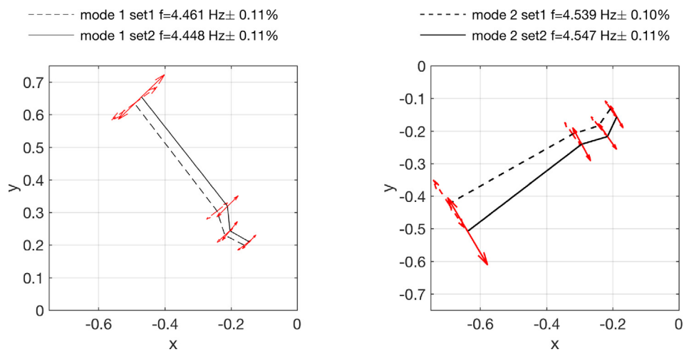
Fig. 12. Eddystone first pair of modes for upper level ordinates.
