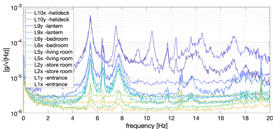
Fig. 5. Les Hanois Lighthouse ambient response power spectral density.
