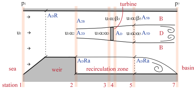
Fig. 4. A schematic sketch of the flow passing a barrage weir and turbine via a streamtube passing the turbine (indicated D ), a bypass streamtube (indicated B ), and a recirculation zone of the weir, driven by a pressure difference ( p_7 - p_1 ). The numbers refer to the stations of the model schematization. The respective velocities within the domain are expressed as a factor times the inflow velocity u_1 (at station 1), using the velocity factors \alpha in the turbine streamtube and \beta in the bypass. The cross-sectional area of a streamtube at each station is expressed as the product of the rotor-swept area A_D , the relative weir area a , and the blockage 1/R . An overview of the velocity and cross section of each streamtube is provided in the supplementary material [23].
