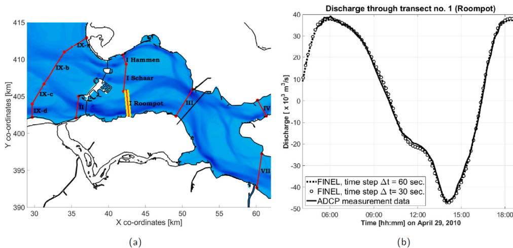
Fig. 7. Calibration of shallow-water flow model; locations of ADCP transects across the Eastern Scheldt basin used for model calibration (a), computed and observed discharge past transect no. I in the Roompot inlet (marked in yellow). (b).
