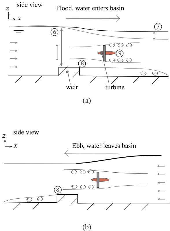
Fig. 2. Schematic overview (side) of turbine-barrage flow interaction at device scale, of \mathcal{O}(1-10) m, during flood flow (a) and ebb flow (b), illustrating the relevant processes: 6. flow contraction by local blockage, 7. free-surface level variation, 8. flow expansion downstream of the weir, 9. flow expansion in the turbine wake.
