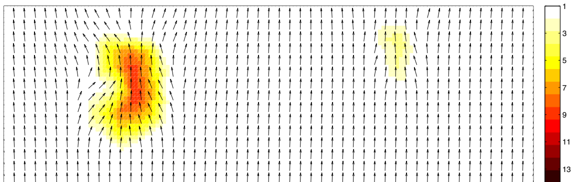
FIGURE 9 Spatial distribution of wave energy (in \text{m}^2 ) and vector plot of mean wave direction obtained with scheme FDM-flux [Colour figure can be viewed at wileyonlinelibrary.com ]
