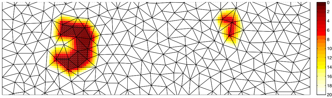
FIGURE 6 A part of the model domain with the bathymetry (in m) projected on the triangular mesh, displaying two submerged shoals [Colour figure can be viewed at wileyonlinelibrary.com ]
