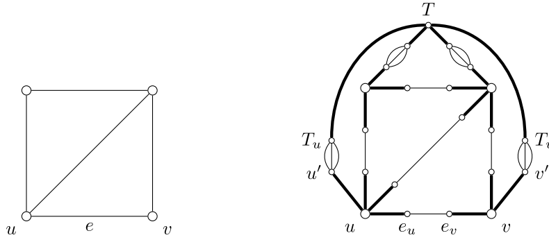
Fig. 4. On the left a graph G , on the right the corresponding graph \widehat{G} , where the M -fold parallel edges are drawn as bold edges. Here M = 12 + 10 + 2 = 24 .
