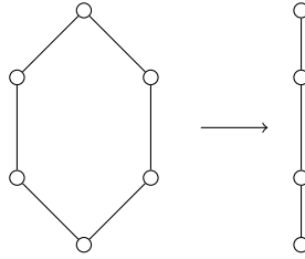
Fig. 3. A finite harmonic morphism from a cycle to a path. Every vertex is mapped to the vertex on its right side and every edge is assigned index 1.
