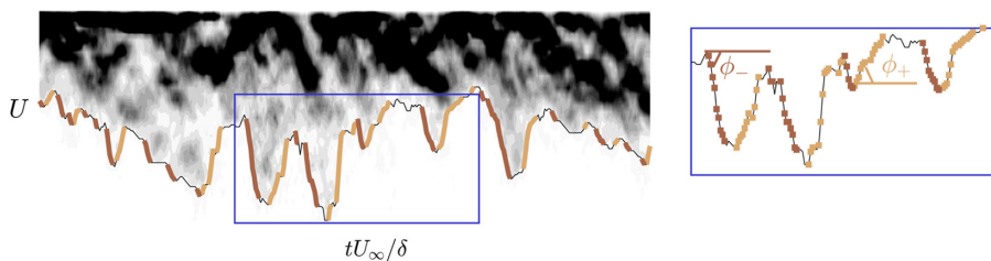
FIG. 3. An illustration of the transitions in \mathcal{P}(U, t) -TRPlV, adapted from Ref. [3]. The identified \phi_+ ( \Delta U_* > 0 , light colors) and \phi_- ( \Delta U_* < 0 , dark colors) transitions of U_* are shown on the left, with the corresponding definitions on the detail on the right.
