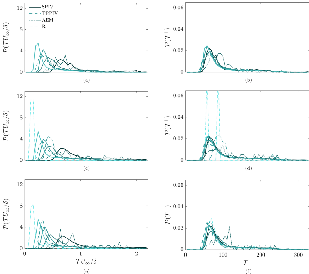
FIG. 10. PDF of \mathcal{T}(U_m) , as defined in Fig. 7. Outer (left) and inner (right) scaling for 0.63 \leq U_m/U_\infty \leq 0.66 (a), (b); 0.72 \leq U_m/U_\infty \leq 0.75 (c), (d); and 0.81 \leq U_m/U_\infty \leq 0.84 (e), (f). Increasing \text{Re}_\tau is denoted with lighter colors.
