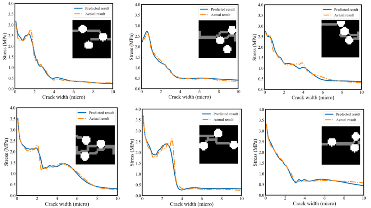
Fig. 17. A randomly chosen set of 6 predicted stress-crack width curves compared to the actual results from lattice model.
