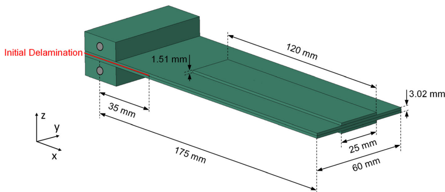
FIGURE 6 R-DCB geometrical dimensions 11 [Colour figure can be viewed at wileyonlinelibrary.com ]
