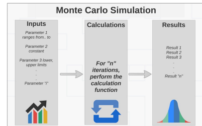
Fig. 1: Monte Carlo Simulation Summary
