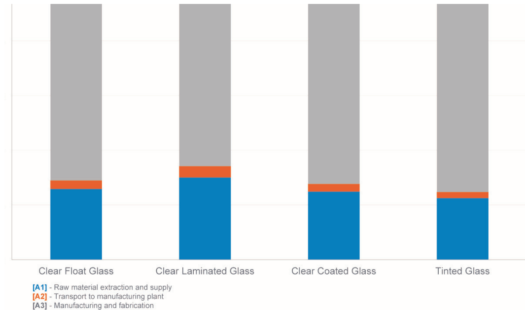
FIG. 4 Results of cradle-to-gate assessment showing a breakdown of embodied emissions for the A1 - A3 phases.
