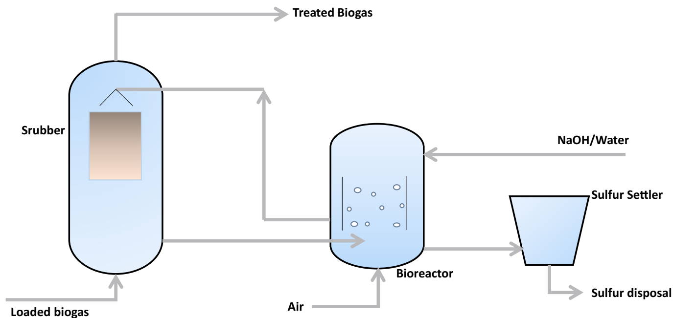
Fig. 4. Schematic flow of Sulfothane desulfurization technology [195].
