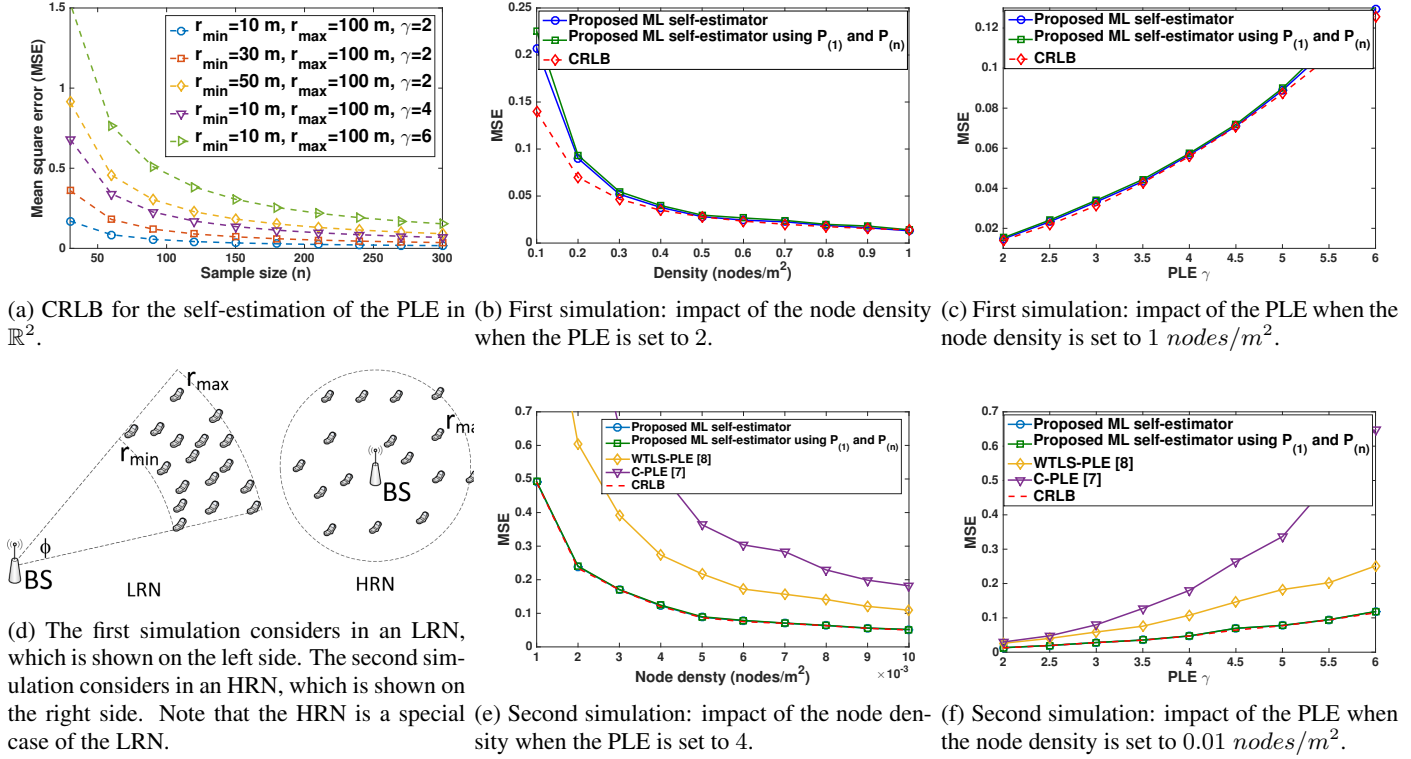
Fig. 3: The simulations assume a 2-dimensional space, where nodes are randomly deployed. The carrier frequency is 2.4 GHz. The transmit power is 1 Watt. The antenna gains G_t and G_r are both 1. For the first simulation, r_{\min} = 50 m, r_{\max} = 100 m and \phi = \pi/6 . For the second simulation, r_{\max} = 100 m.
