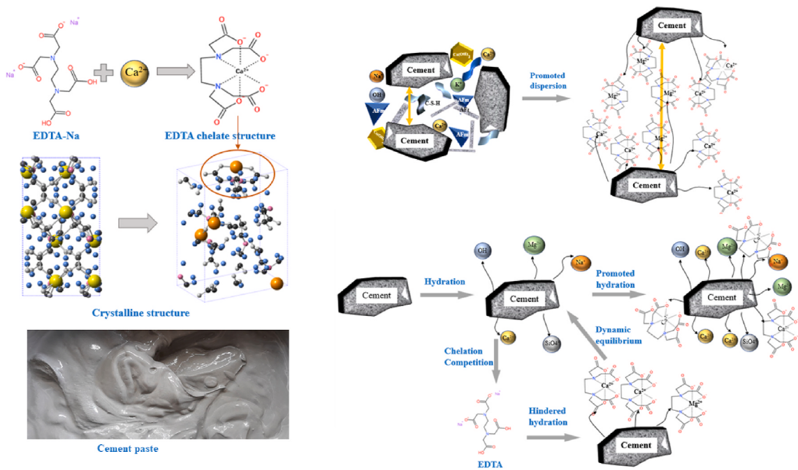
Fig. 14. Mechanism of EDTA on the hydration of cement paste.
