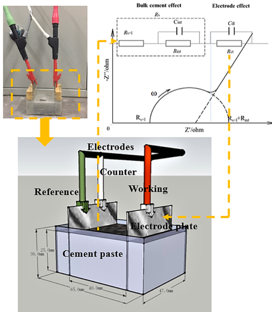
Fig. 2. Classic Nyquist model and equivalent circuit of the electrode-cement paste system.
