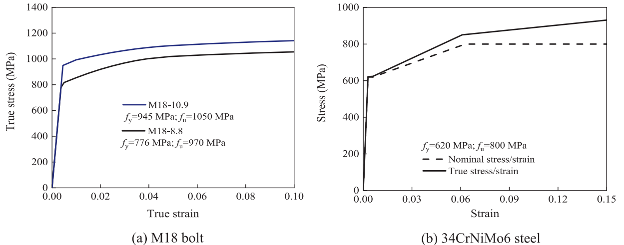
Fig. 12. Stress–strain curves for materials used in the bolt and machined components.
