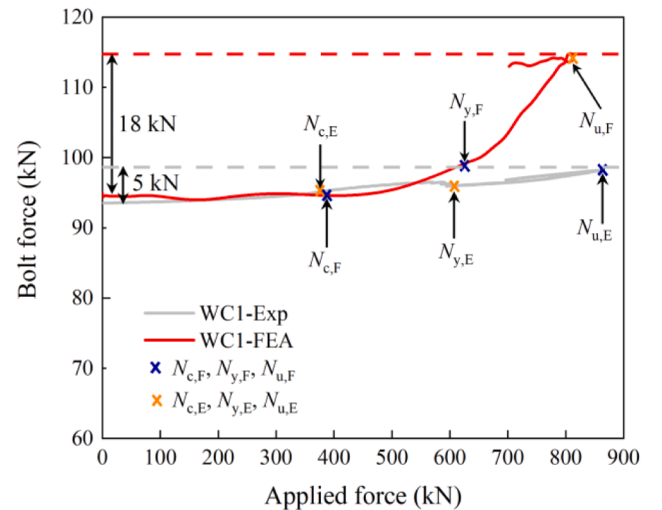
(b) FEA vs. Exp
