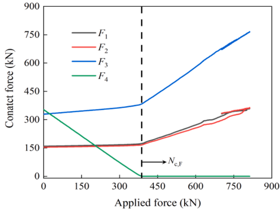
(a) Contact force response of WC1
