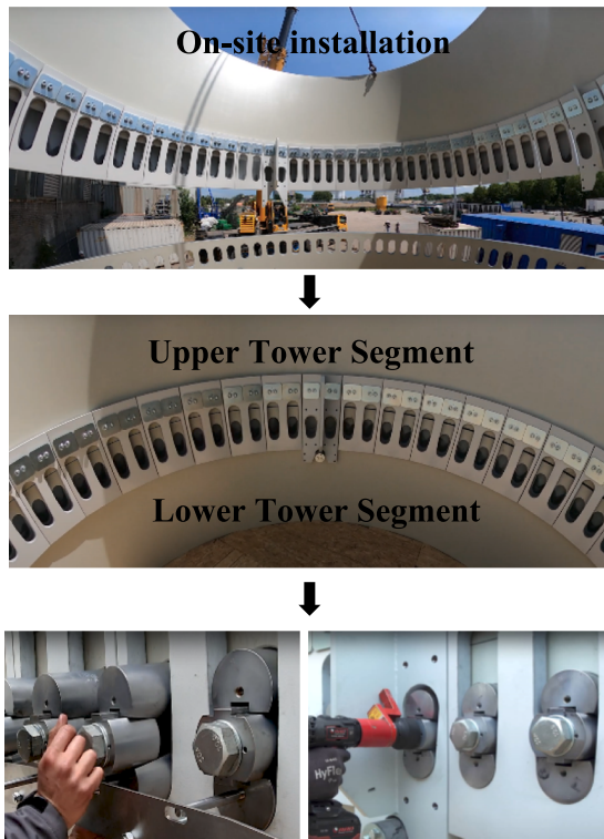
Fig. 2. Performed full-scale tests in OFWEC3 project [23].
