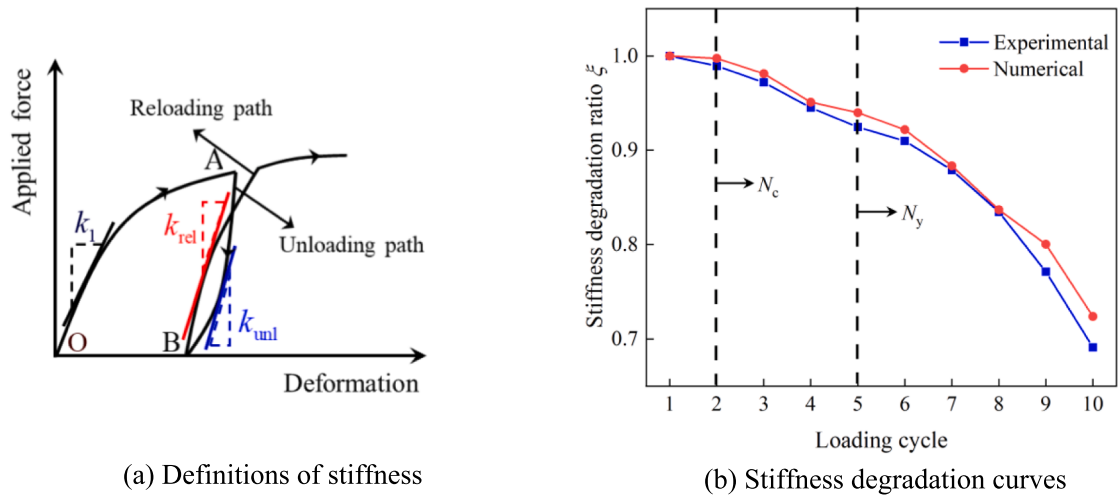
Fig. 25. Evolution of stiffness degradation with the number of cycles.
