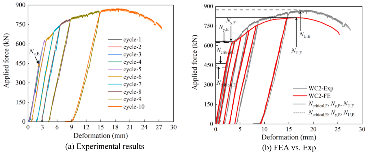
Fig. 24. Load-displacement curves of WC2.
