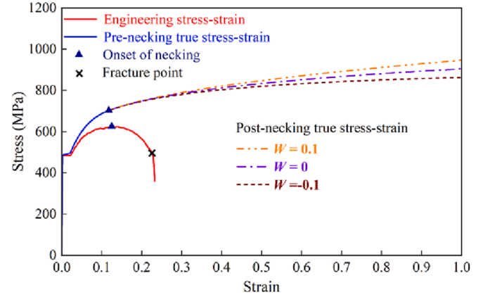
Fig. 10. Full-range stress–strain relationship of S460 steel.
