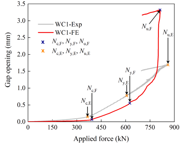
(b) FEA vs. Exp
