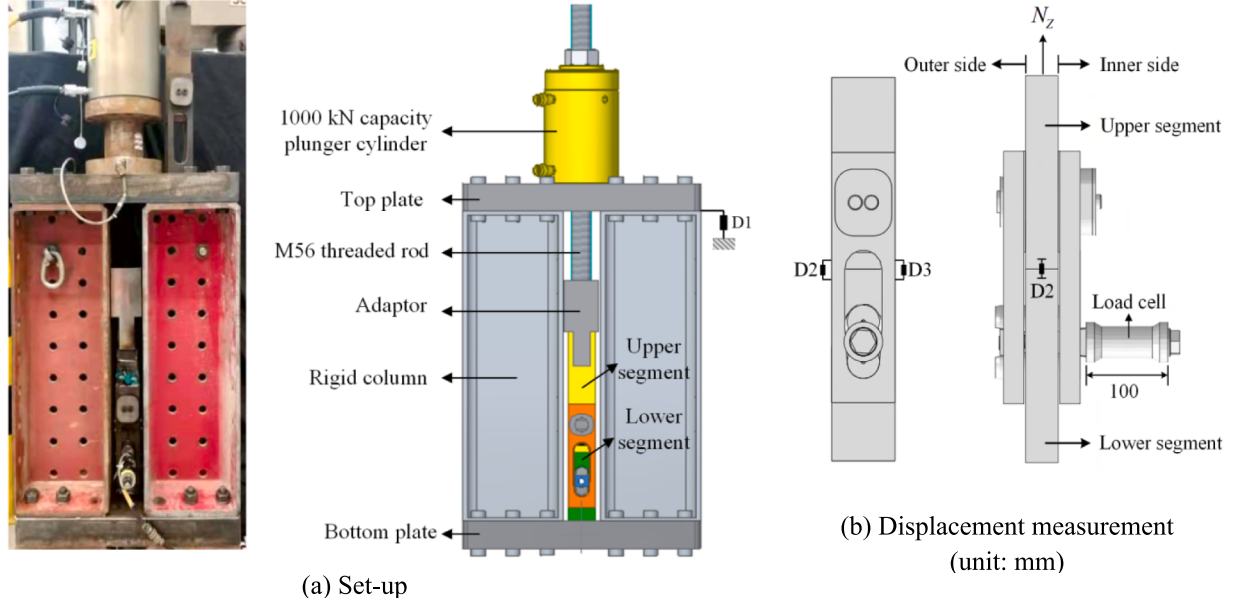
Fig. 6. Experimental system.
